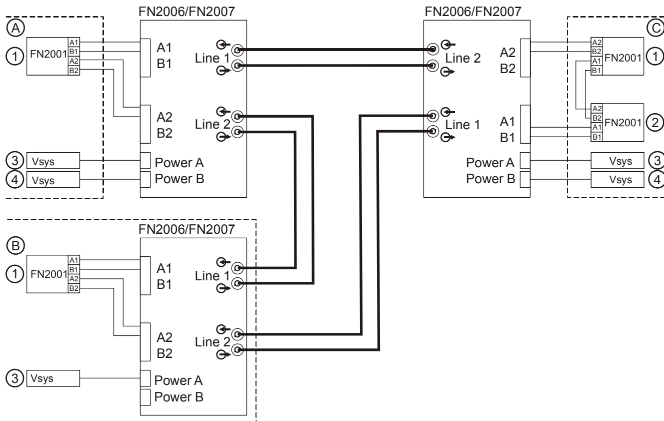
Figure 37: Example of different wirings of the fiber optic cable network module
