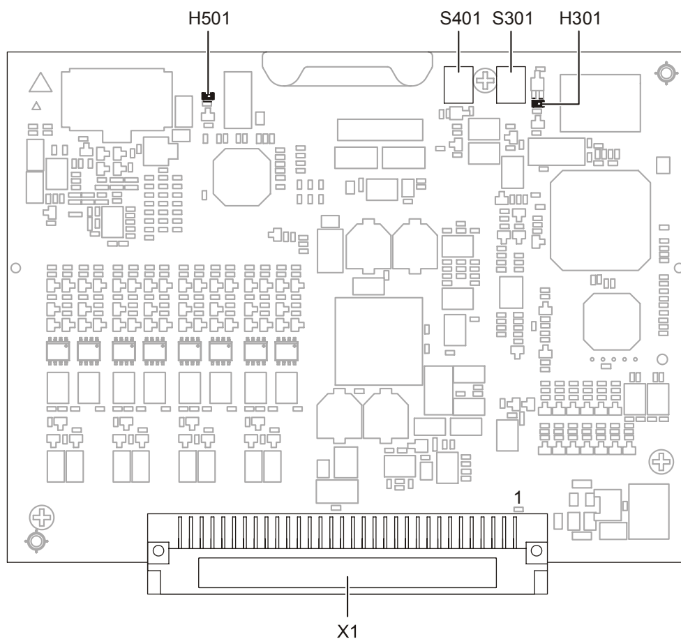
Figure 54: Printed circuit board view of line card (FDnet / C-NET) FCL2001-A1
