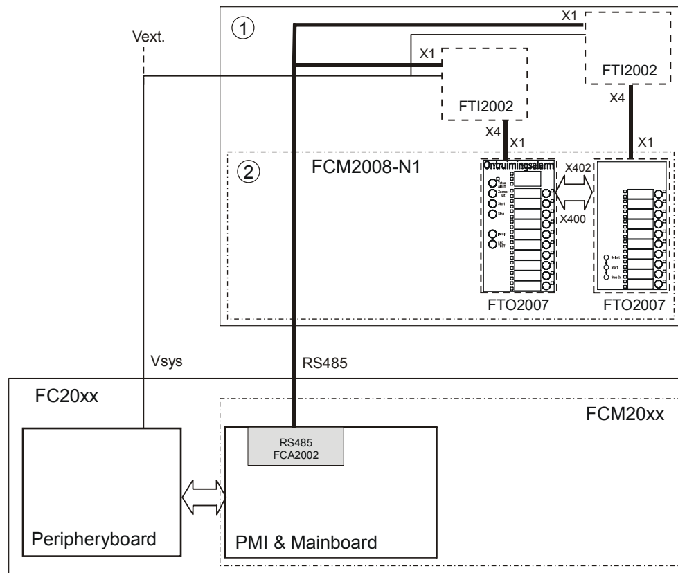
Figure 107: Wiring of the EVAC-NL connector board FTI2002-N1 in a remote EVAC 20-zone indicator
