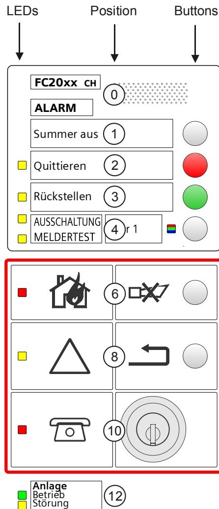
Figure 23: Layout of front panel for FT2080-C2
