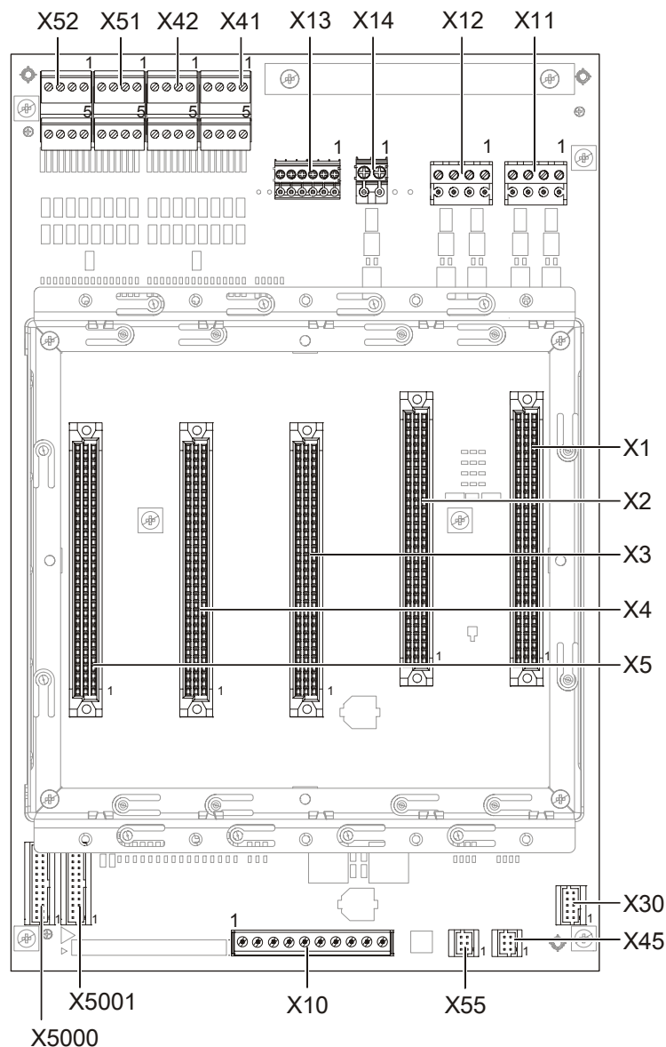
Figure 72: Printed circuit board view of card cage (CPU) FCC2003-A1
