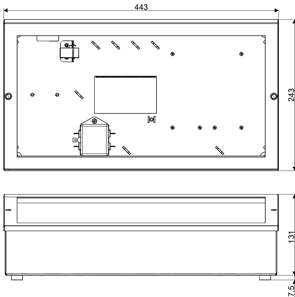
Figure 93: Dimensioned drawing of desktop housing (FT2080) FHA2040-A1, with cover
