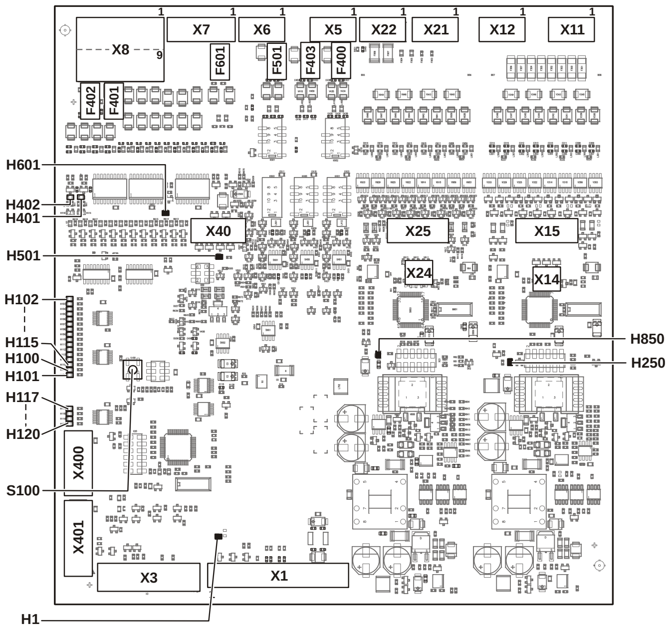
Figure 14: Printed circuit board view FCI2004
