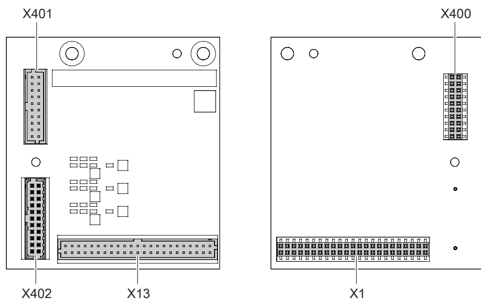
Figure 43: Connection module (MoNet) FCA2031, printed circuit board view of front and rear panels
