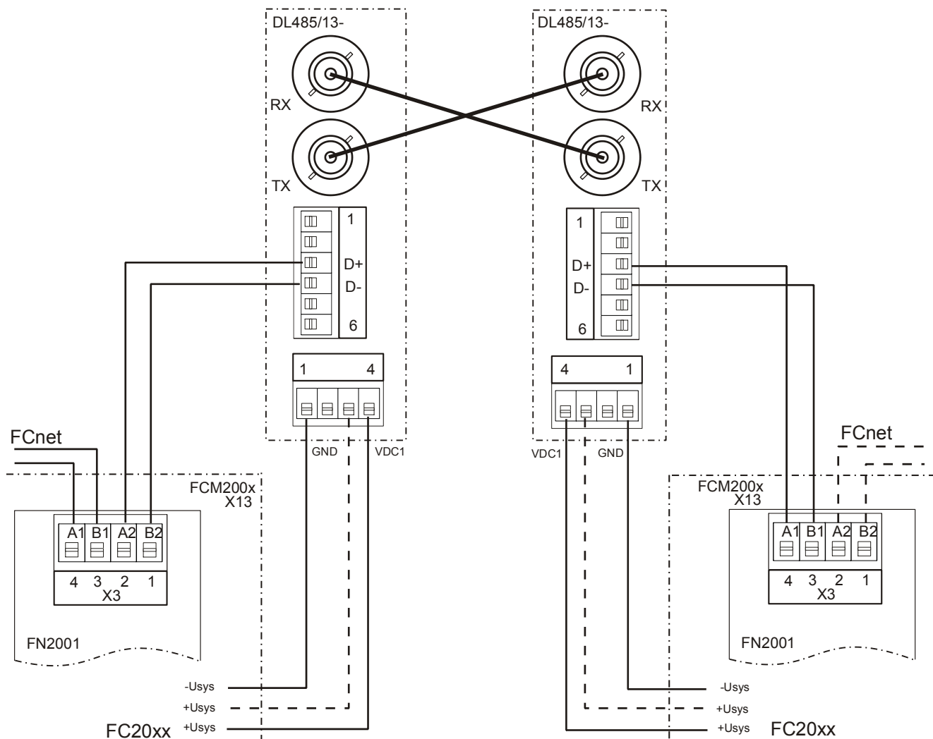
Figure 46: Wiring the interface module DL485/13-MM-ST-SBT
