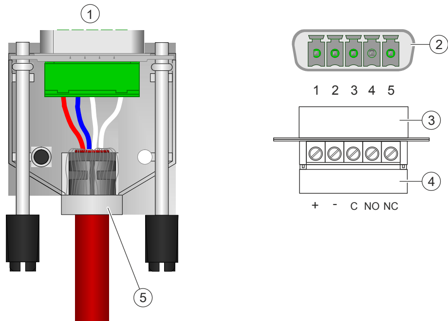
Figure 34: Connector for Power A and Power B sockets
