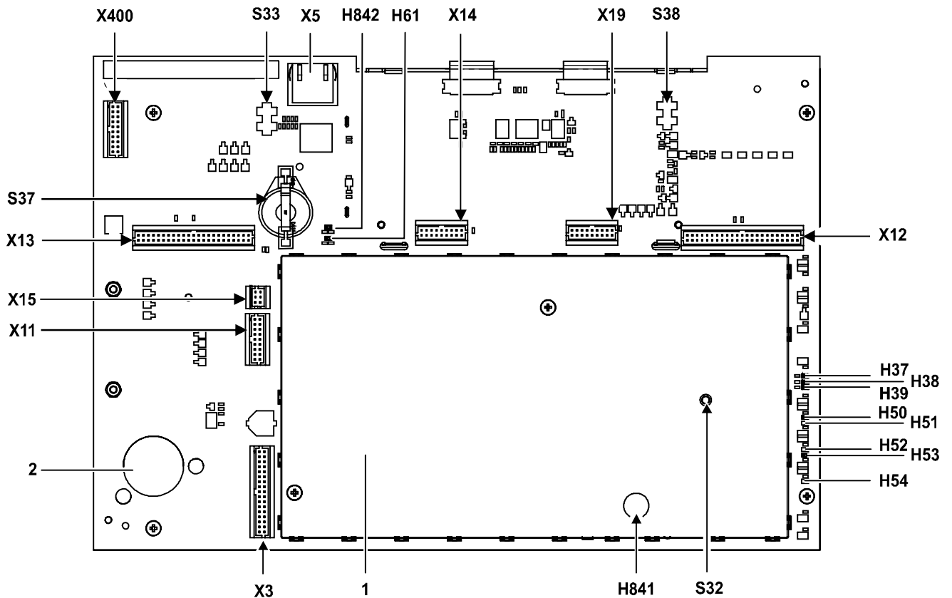
Figure 17: Equipment for PMI & mainboard FCM2027
