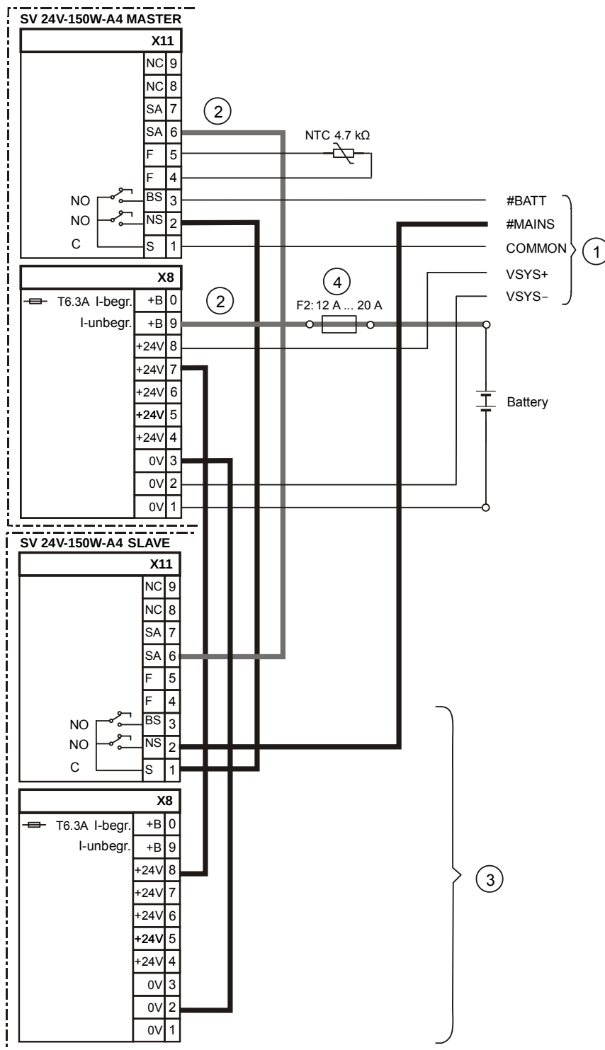
Figure 5: Parallel connection of two power supplies (150 W)-A4
