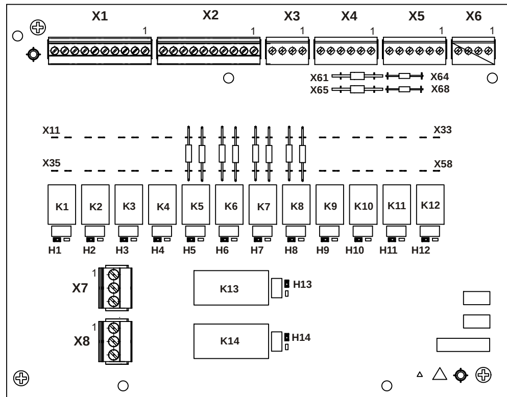
Figure 116: Printed circuit board display RT Interface FCI2005
