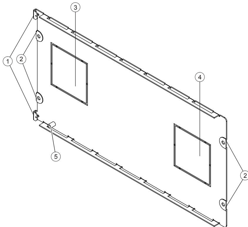
Figure 81: Carrier plate, interior view
