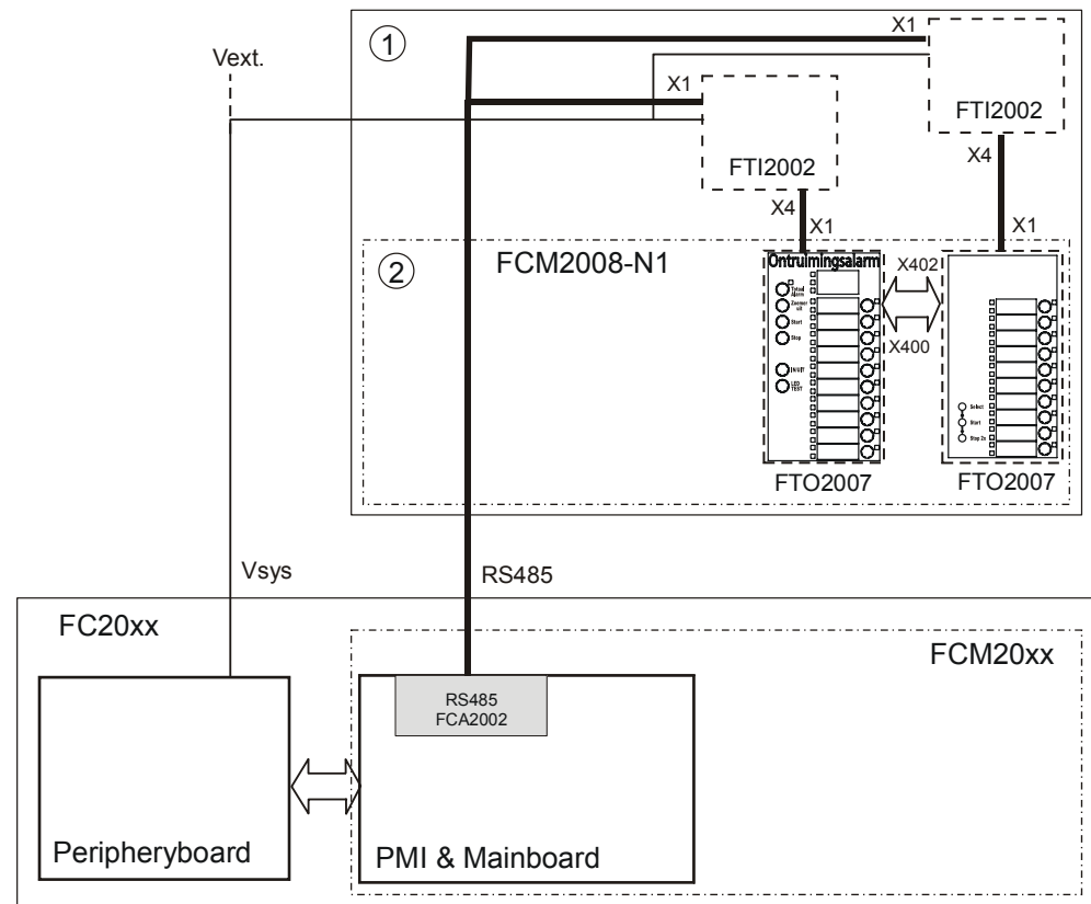
Figure 104: Wiring of the remote EVAC 20-zone display via the RS485 interface
