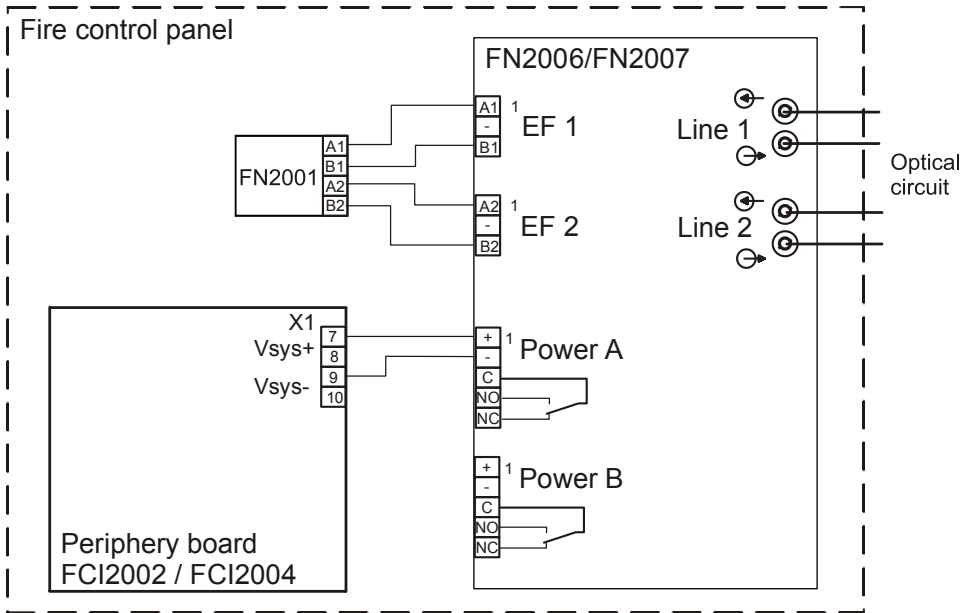
Figure 36: Example of wiring the FN2006 / FN2007 to the FN2001 for internal installation
