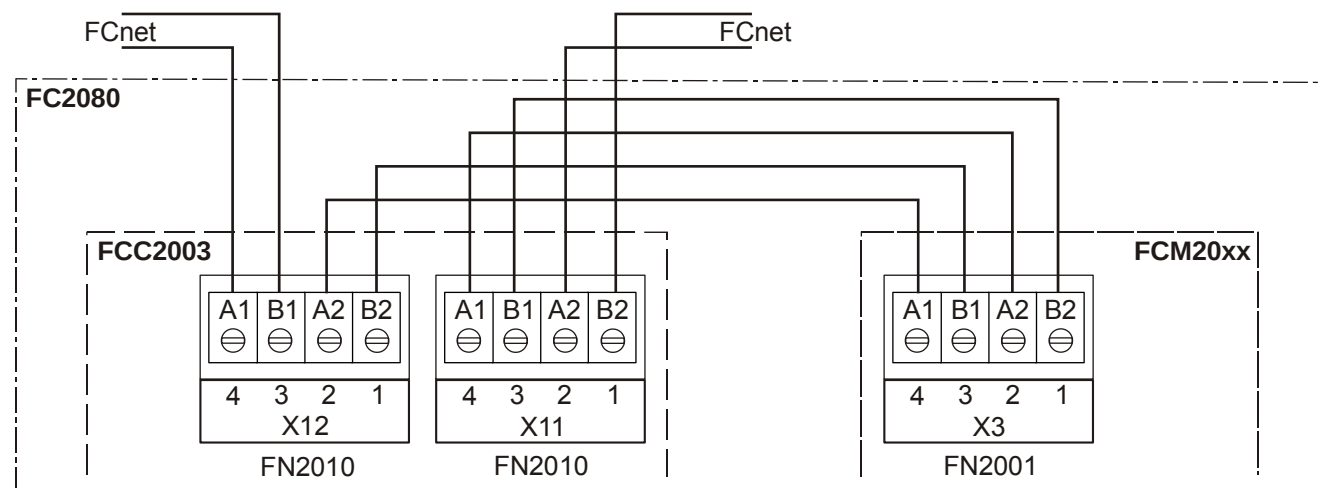
Figure 74: ↑ FCnet networking of FG2020 with optional operating unit
