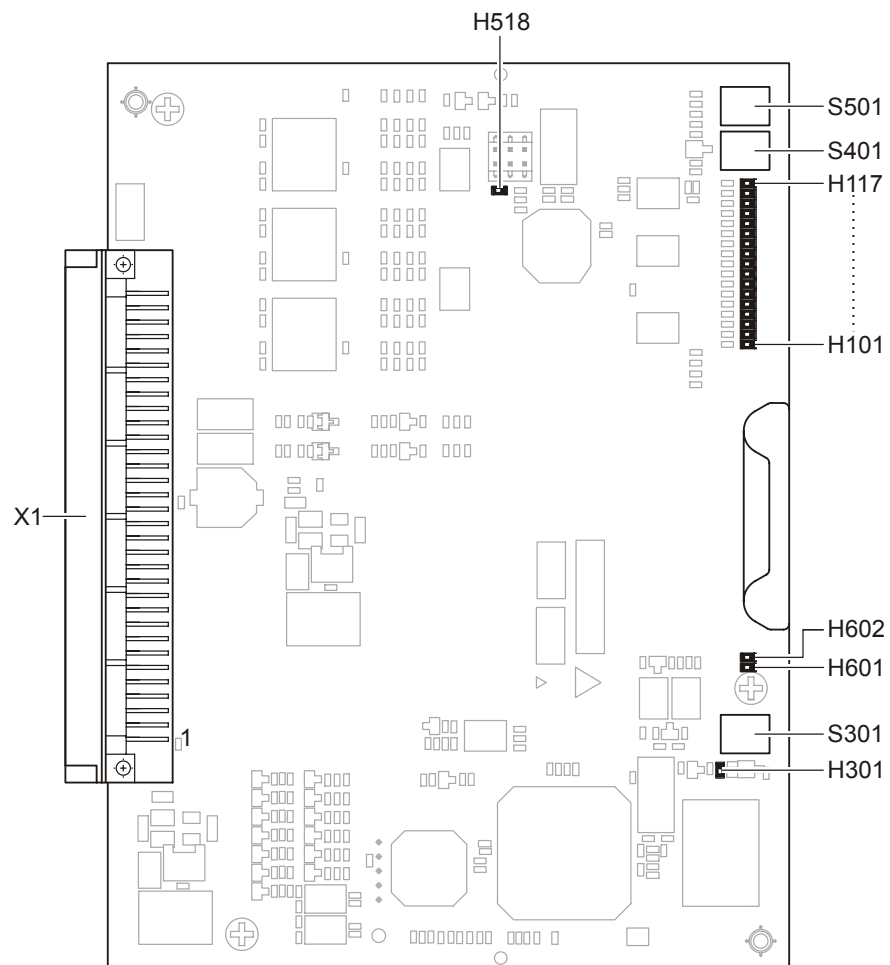
Figure 60: Printed circuit board view I/O card FCI2008-A1
