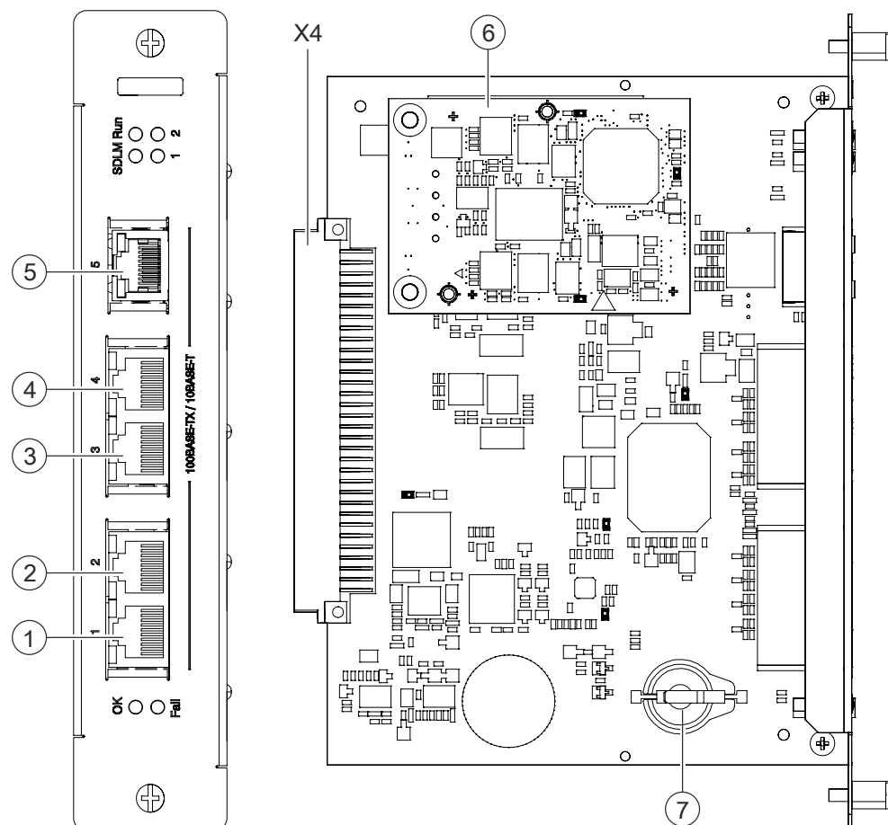
Figure 79: Communication card (FG2020), front and PCB view
