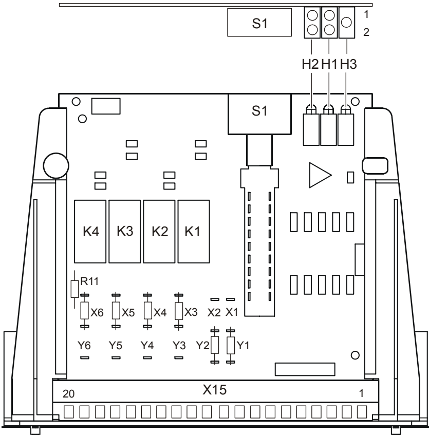
Figure 118: Printed circuit board view of E3G091 (FCI2006-C1 set), view installed and from above
