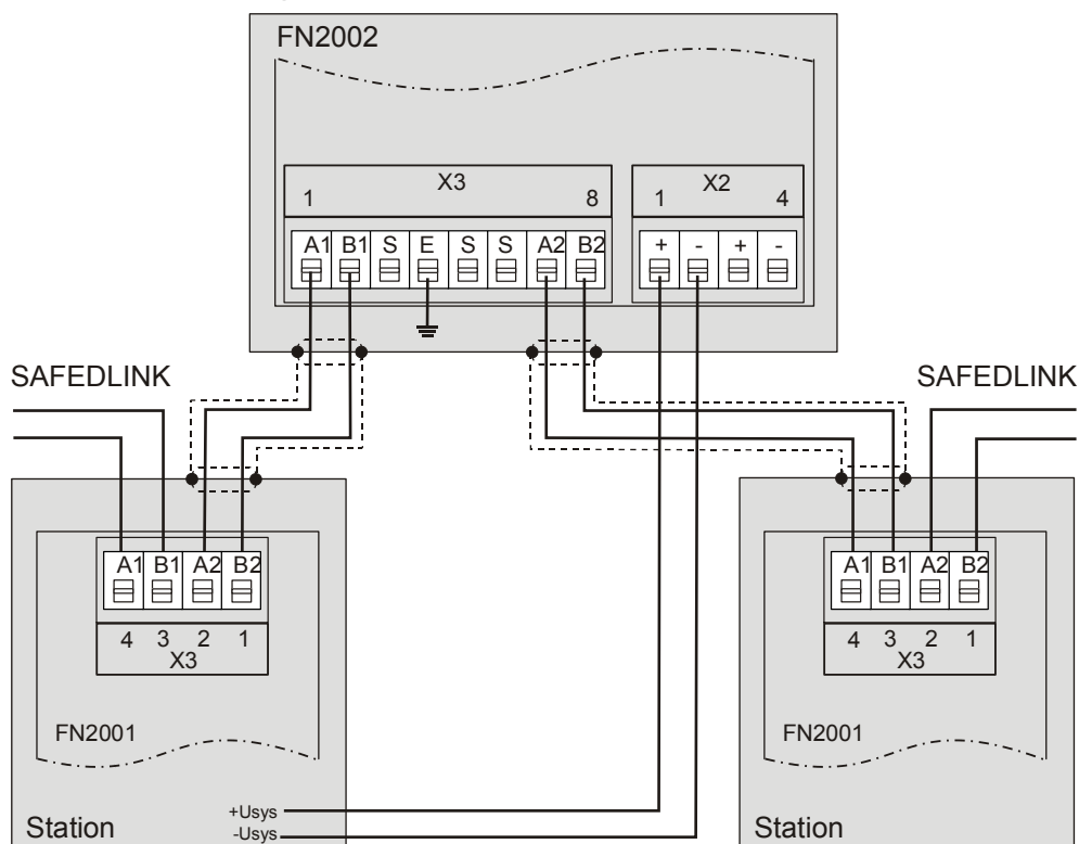
Figure 39: Repeater FN2002, SAFEDLINK wiring
