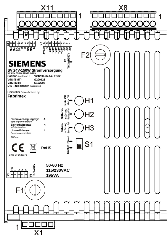
Figure 3: View of the power supply (150 W) SV 24V-150W-A4
