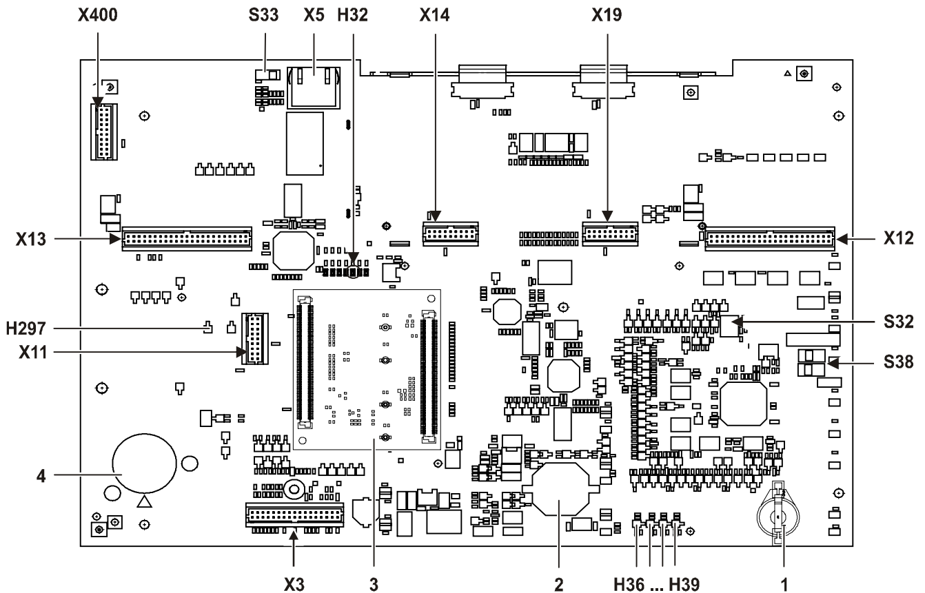
Figure 16: Printed circuit board view of PMI & mainboard
