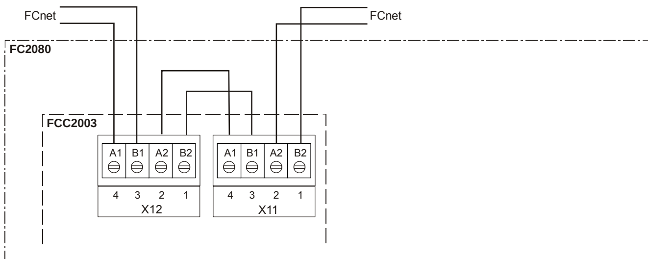
Figure 73: ↑ FCnet networking of FG2020 without operating unit
