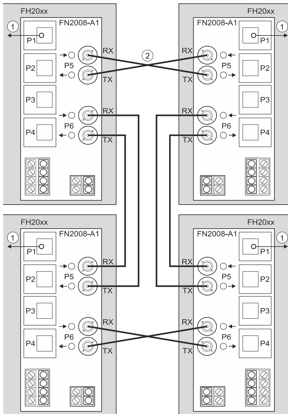
Figure 47: Connecting a fiber optic cable for optical Ethernet with FN2008-A1
