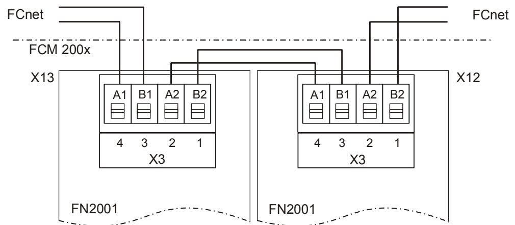
Figure 30: Wiring of 2 network modules
