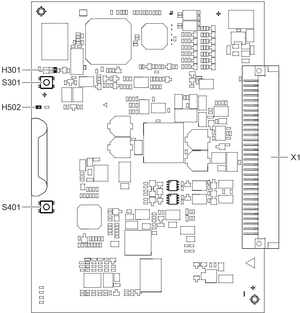
Figure 58: PCB view of the line card (interactive) FCL2006
