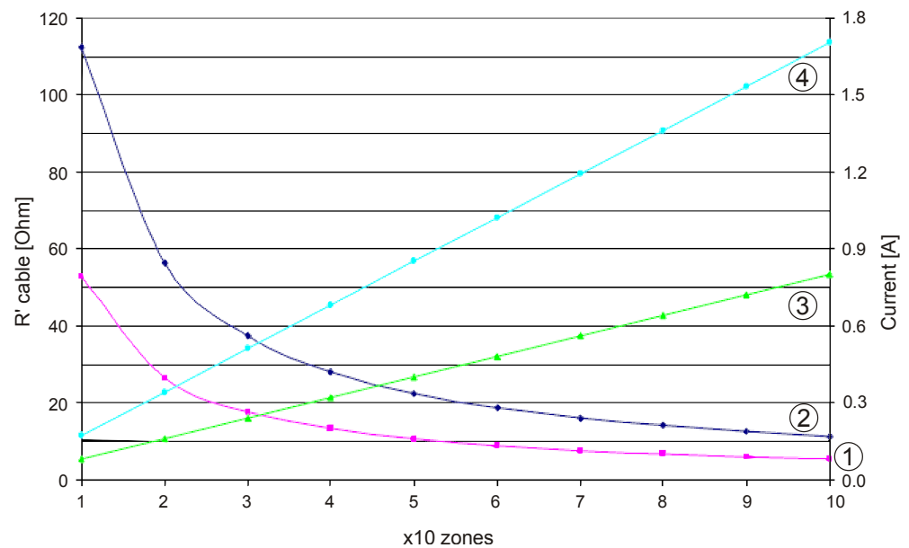
Figure 109: Diagram for calculating the max. cable resistance
