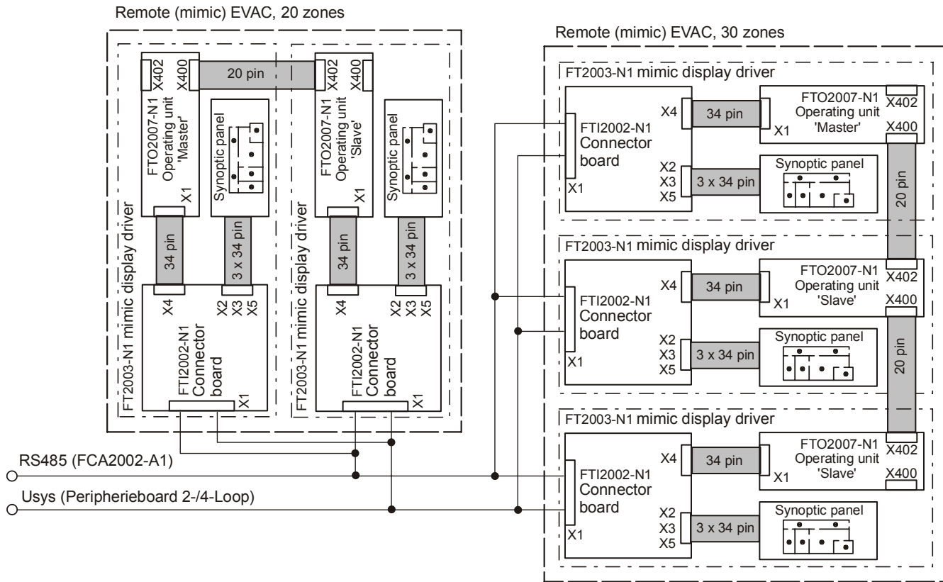
Figure 114: Wiring example for calculating the cable resistance
