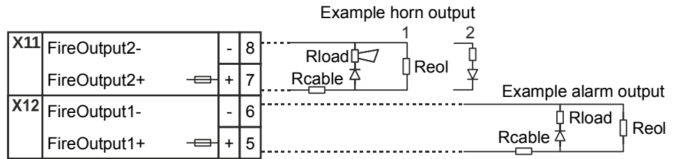
Figure 61: Switching examples for monitored alarm and horn outputs with decoupled load (EN 54)
