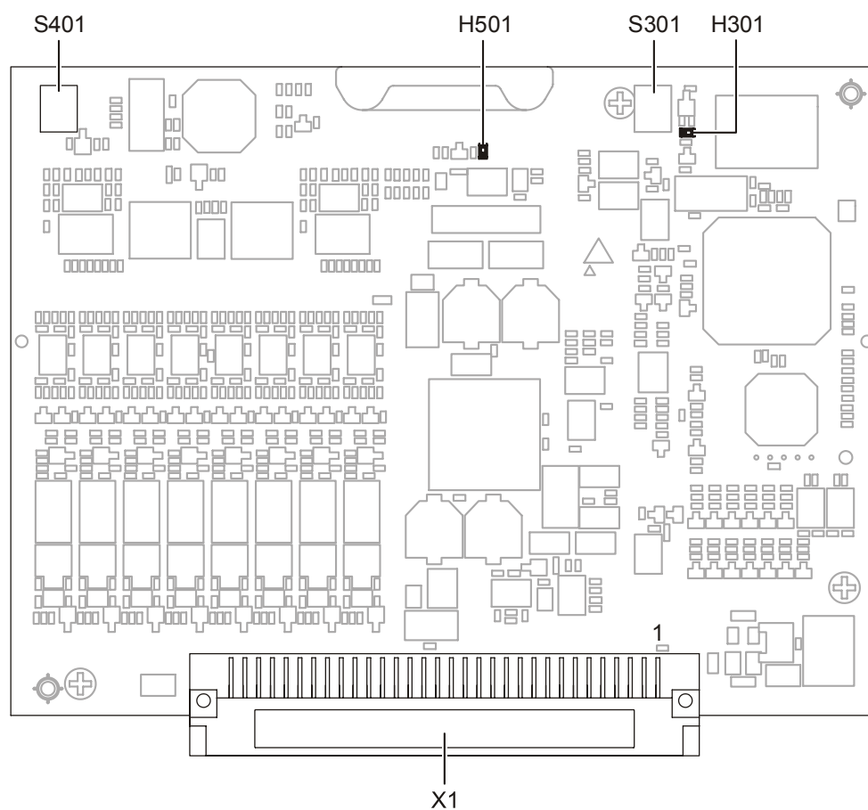
Figure 55: PCB view of line card (collective) FCL2002-A1
