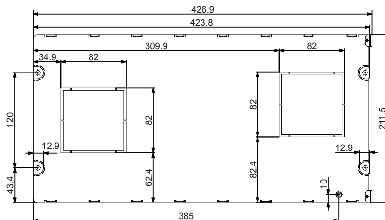
Figure 82: Carrier plate dimensions
