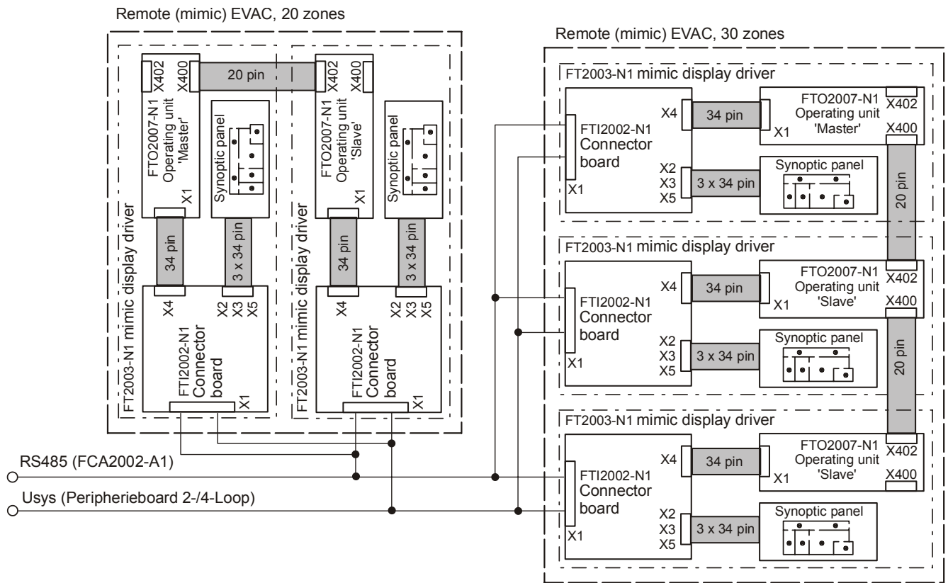
Figure 110: Wiring example for calculating the cable resistance
