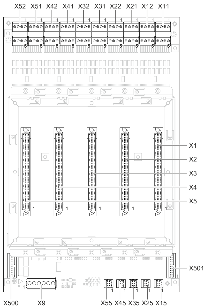
Figure 52: PCB view of card cage (5 slots) FCA2008-A1
