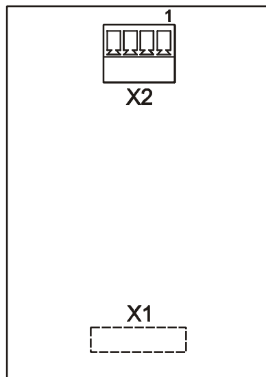
Figure 27: Printed circuit board view of RS485 module (isolated) FCA2002-A1
