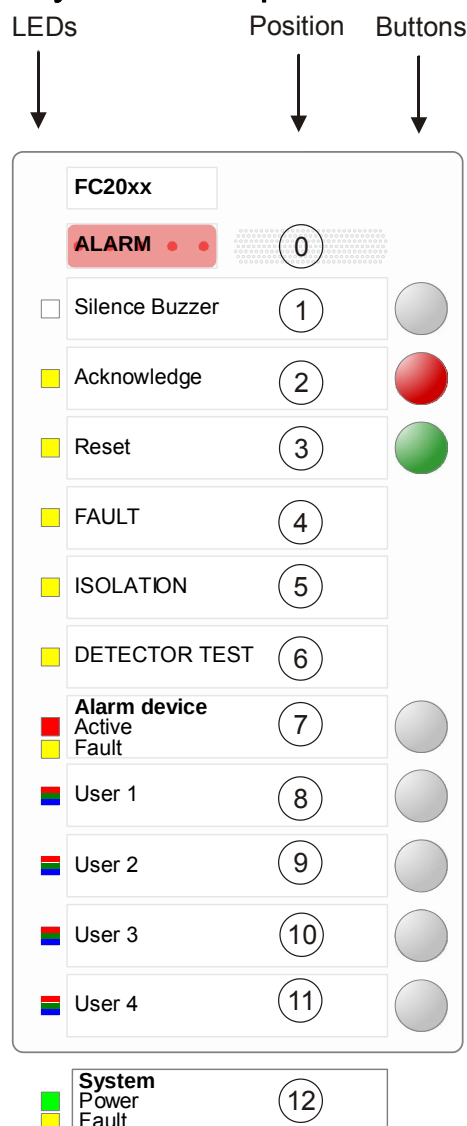
Figure 22: Layout of front panel for FT2080-A1
