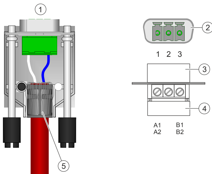
Figure 35: Connector for EF1/EF2 socket, for SAFEDLINK networking
