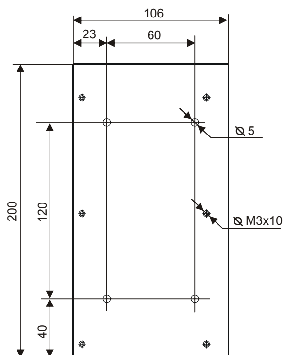
Figure 98: Dimensions of carrier plate for FT2001
