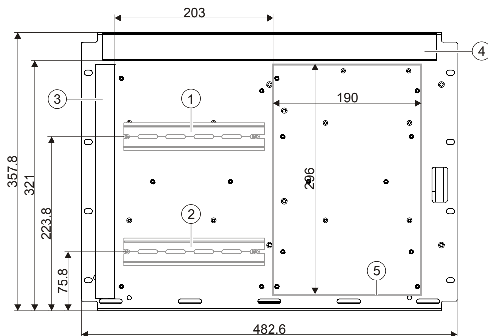
Figure 86: Dimensional drawing of the carrier (19", card cage) FHA2023-A1
