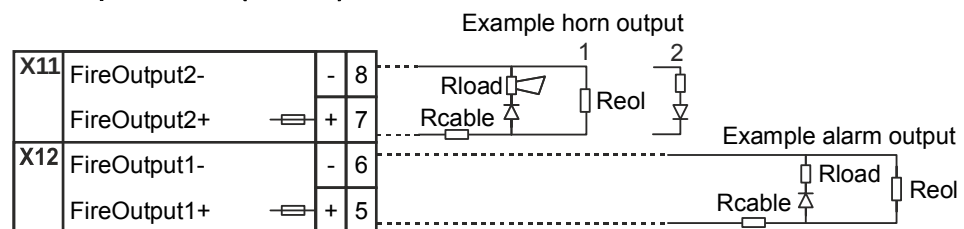
Figure 66: Switching examples for monitored alarm and horn outputs with decoupled load (EN 54)
