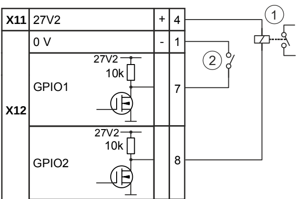
Figure 68: Switching for relays
