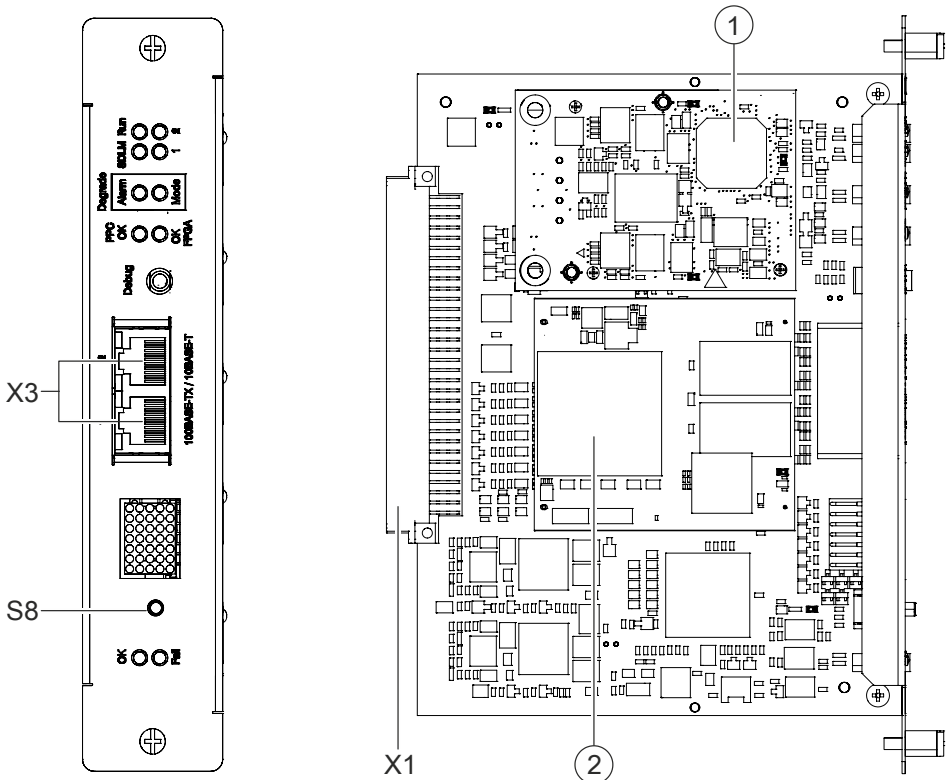
Figure 75: Operating elements, plugs, and modules of the ↑ CPU card (FC2080)
