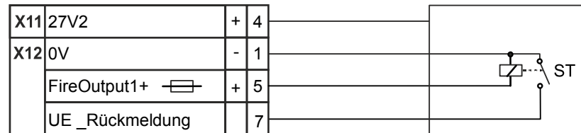
Figure 64: Switching for RE response in accordance with VdS
