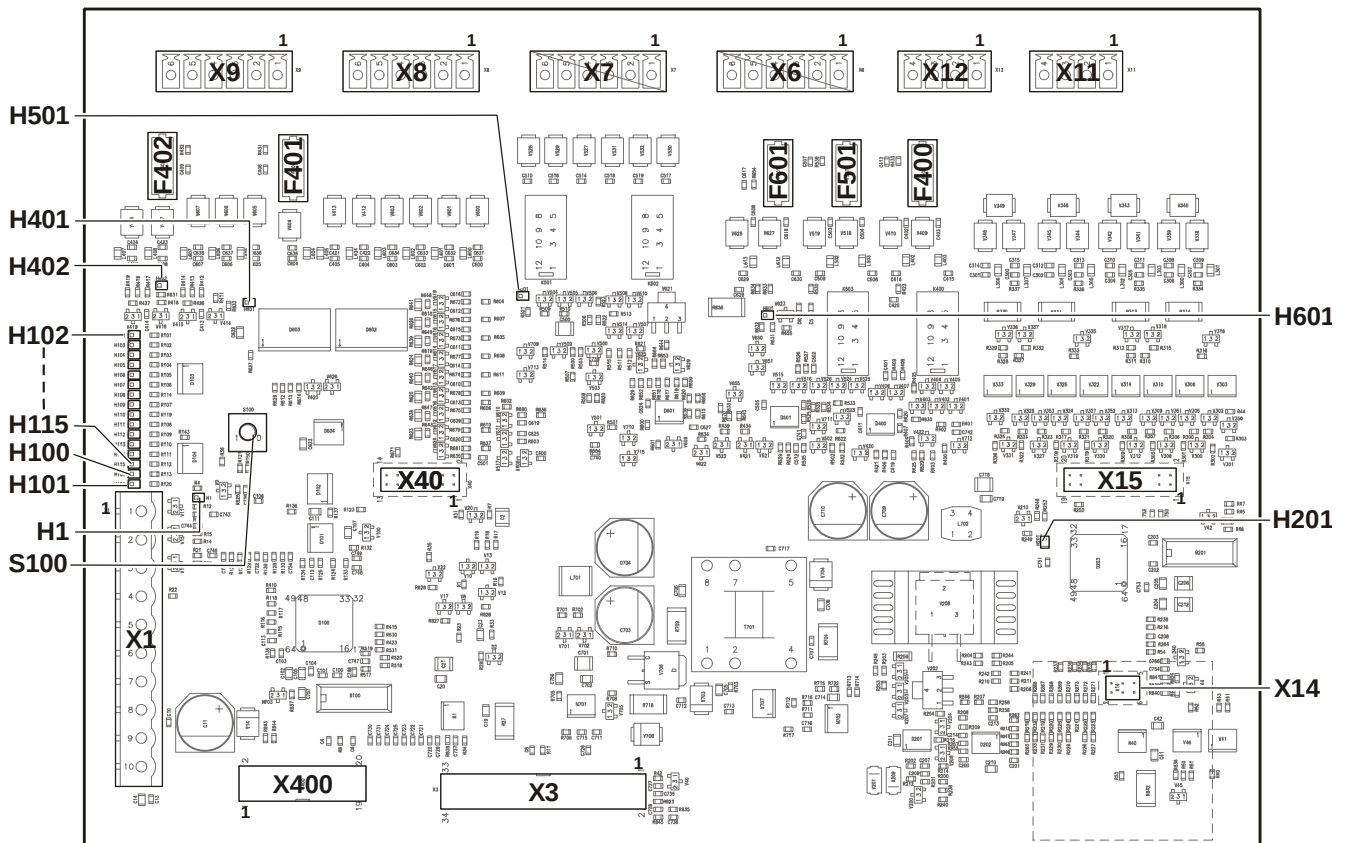
Figure 13: Printed circuit board view of periphery board (2 loops) FCI2002
