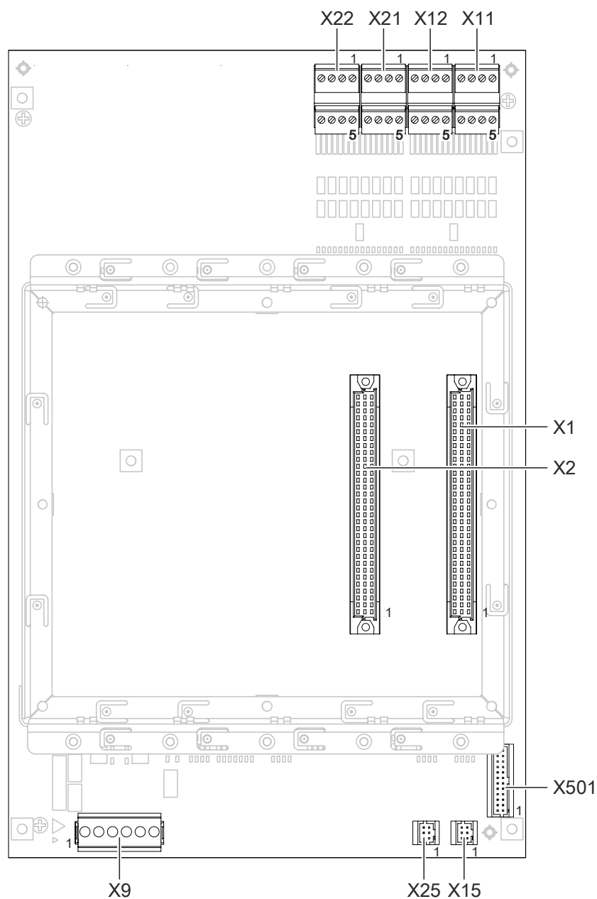
Figure 51: PCB view of card cage (2 slots) FCA2007-A1
