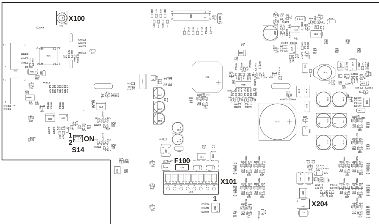
Figure 96: Printed circuit board view of ↑ floor repeater display FT2011
