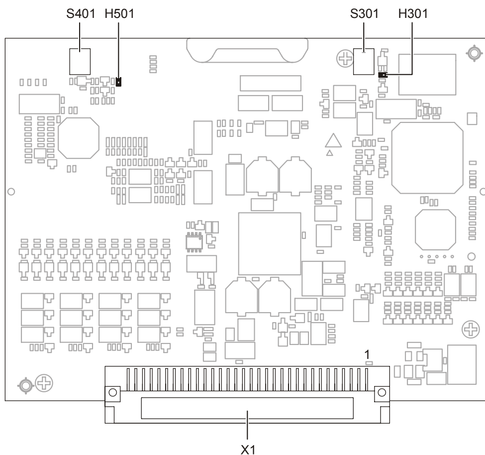
Figure 56: PCB view of line card MS9i FCL2003-A1
