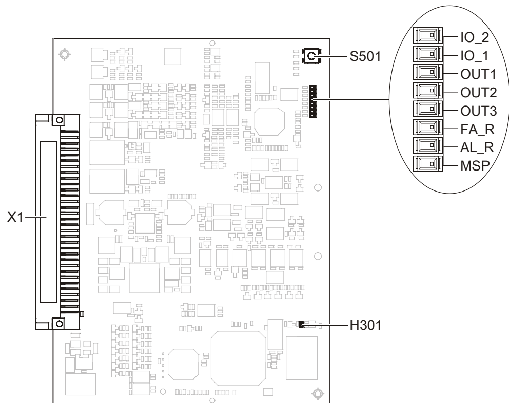
Figure 63: Printed circuit board view I/O card (RT) FCI2007-A1
