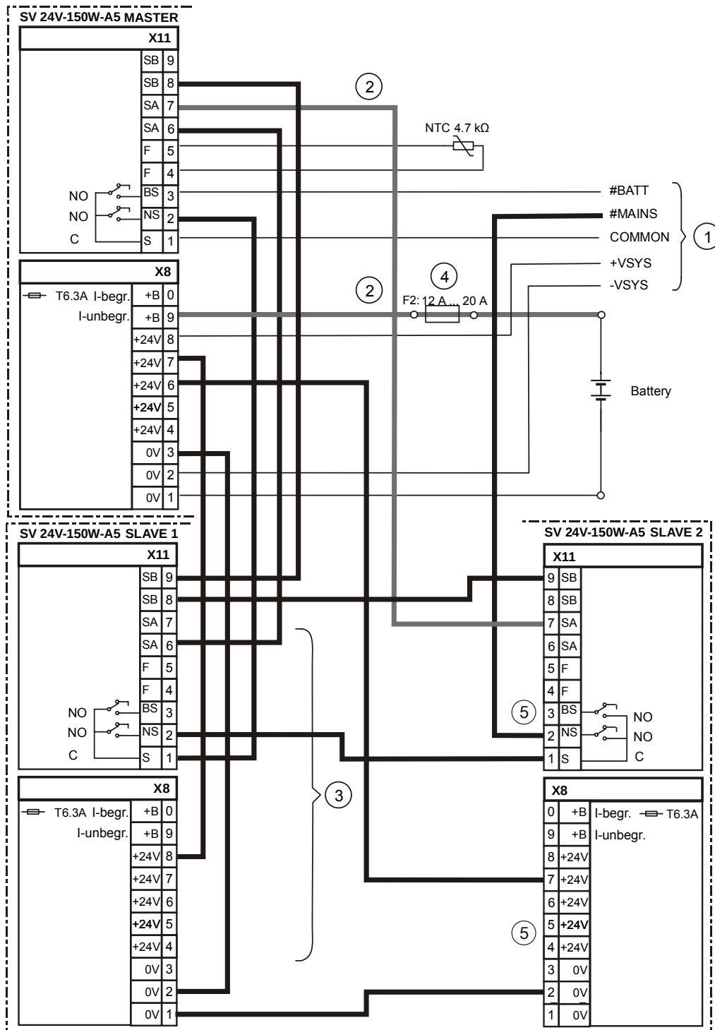
Figure 9: Parallel switching of three power supply units (150 W)-A5
