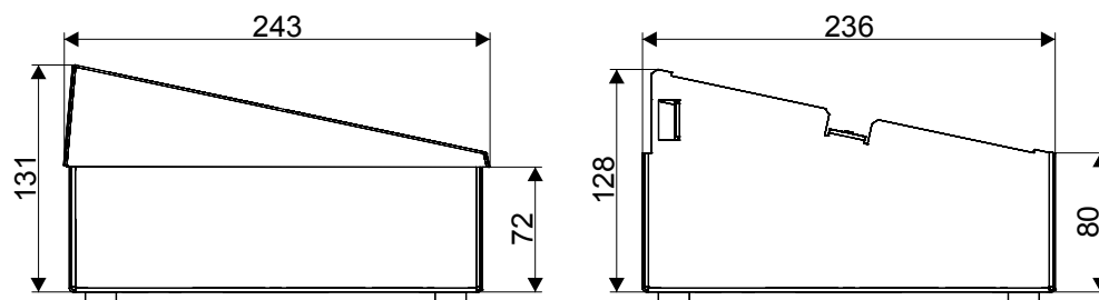
Figure 94: Dimensioned drawing of desktop housing (FT2080) FHA2040-A1, side view with and without cover
