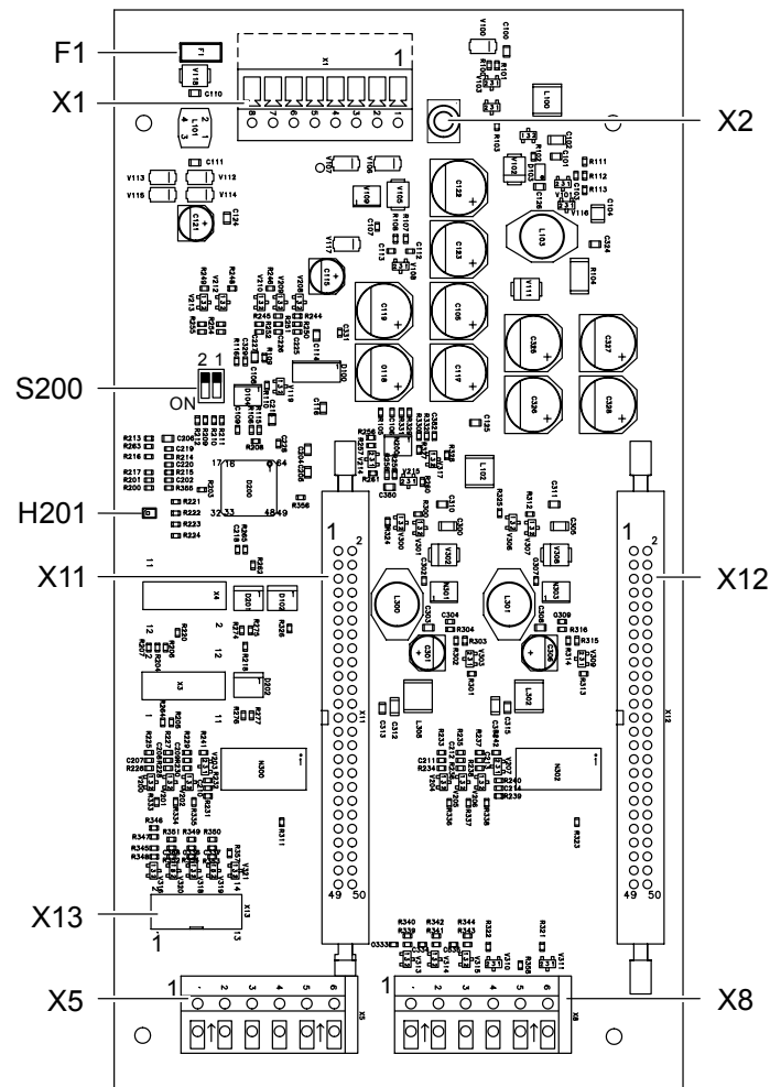
Figure 97: Printed circuit board view FT2001-A1
