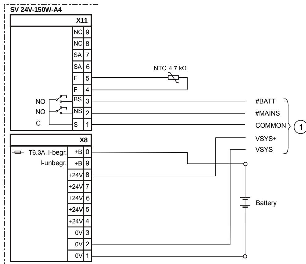
Figure 4: Wiring of the single power supply SV 24V-150W-A4
