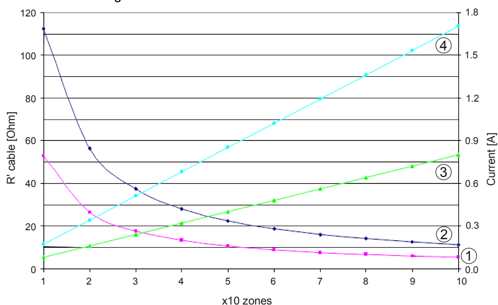
Figure 113: Diagram for calculating the max. cable resistance
