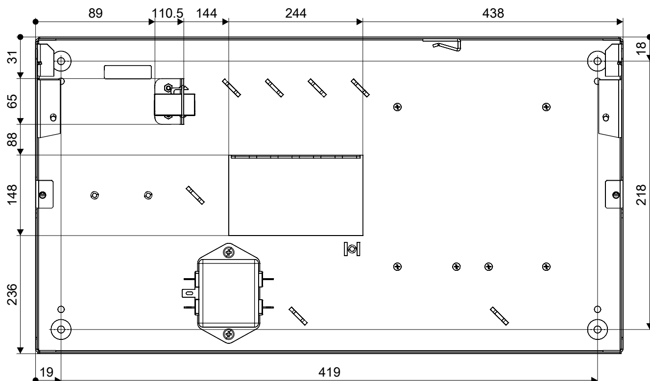
Figure 92: Dimensioned drawing of desktop housing (FT2080) FHA2040-A1, without cover
