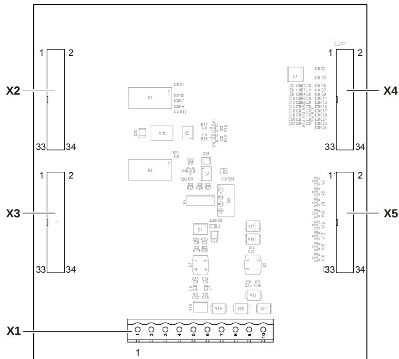
Figure 106: Printed circuit board view of EVAC-NL connector board FTI2002-N1
