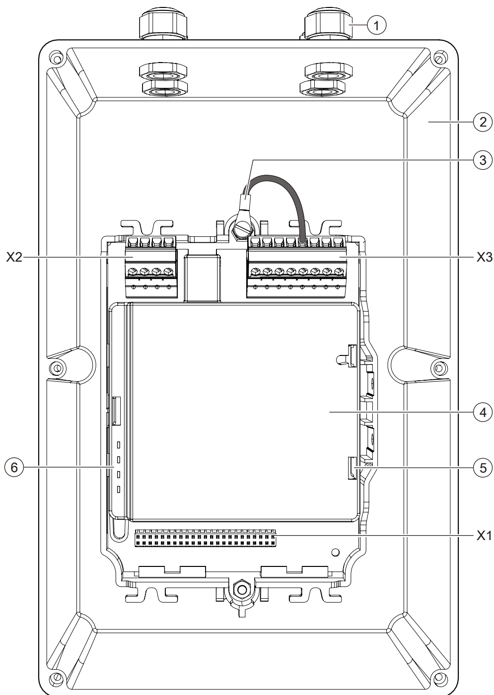
Figure 38: View of repeater, housing open
