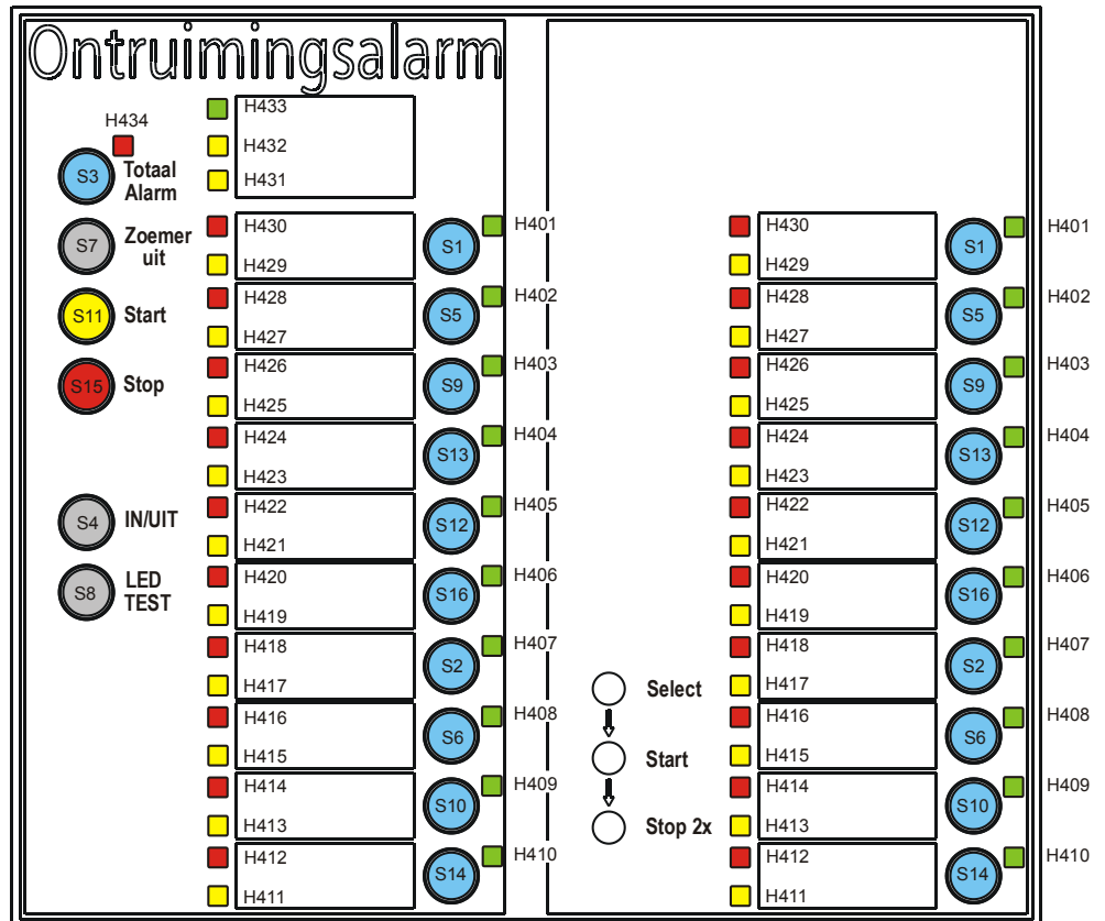
Figure 105: EVAC master unit (left), EVAC slave unit (right)
