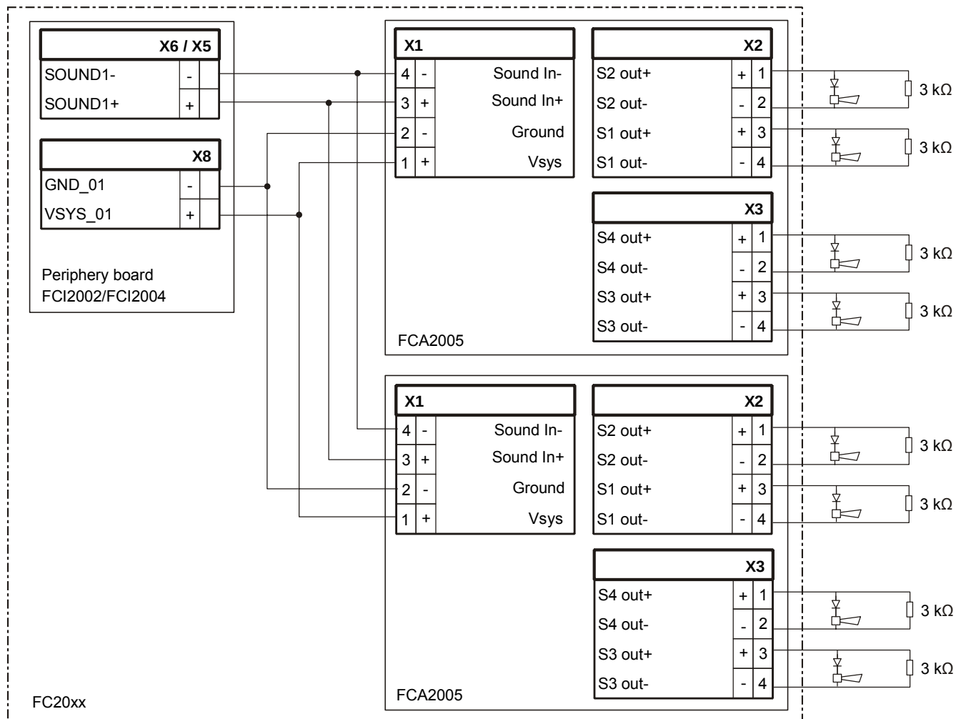
Figure 71: Cascading of two sounder modules FCA2005-A1
