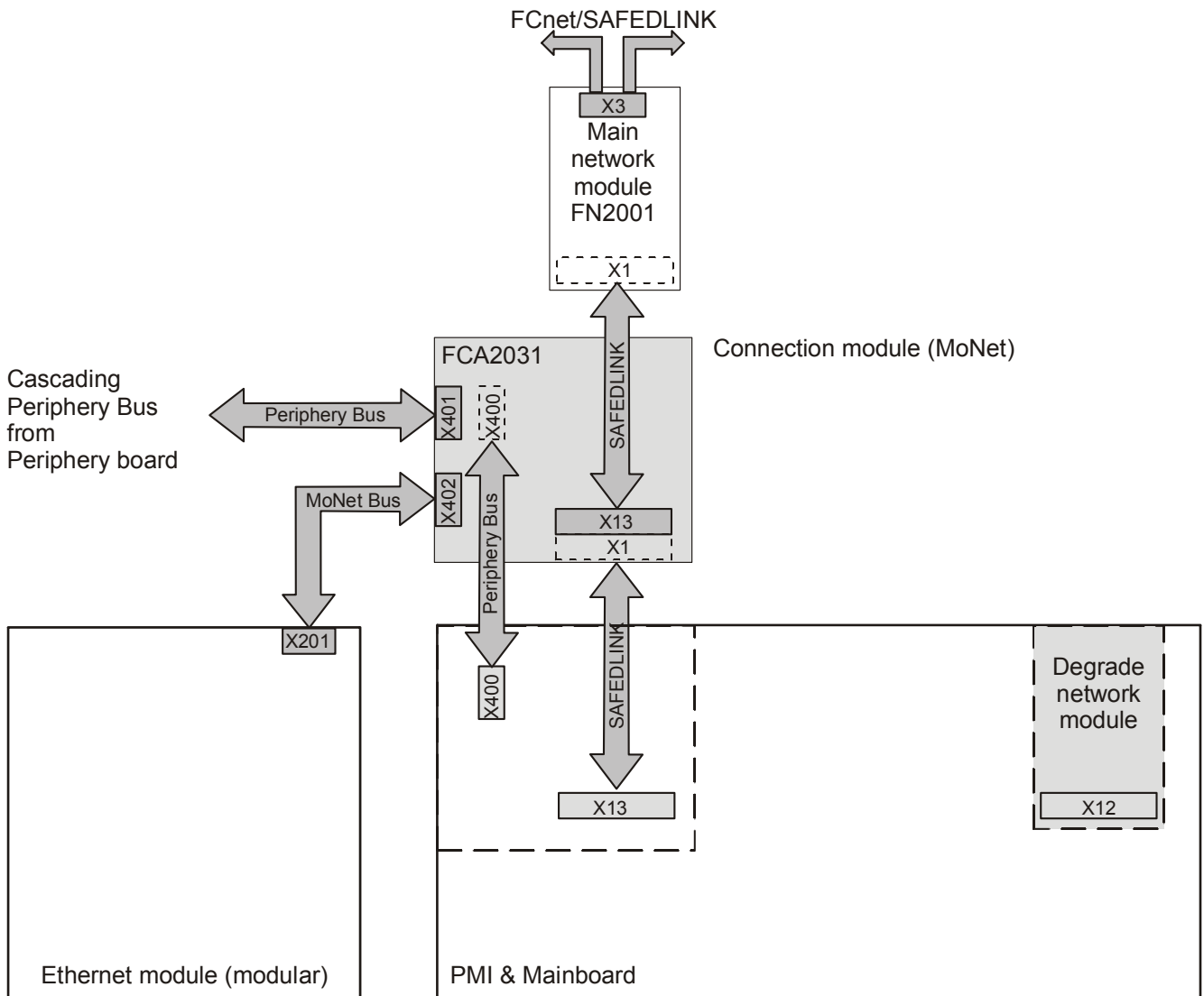
Figure 44: Simplified circuit diagram for connection module (MoNet) FCA2031-A1
