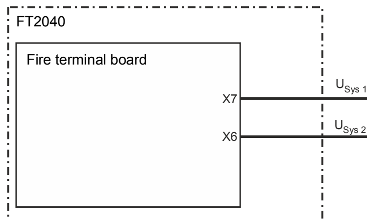
Figure 12: FTI2001-A1, supply via a fire control panel
