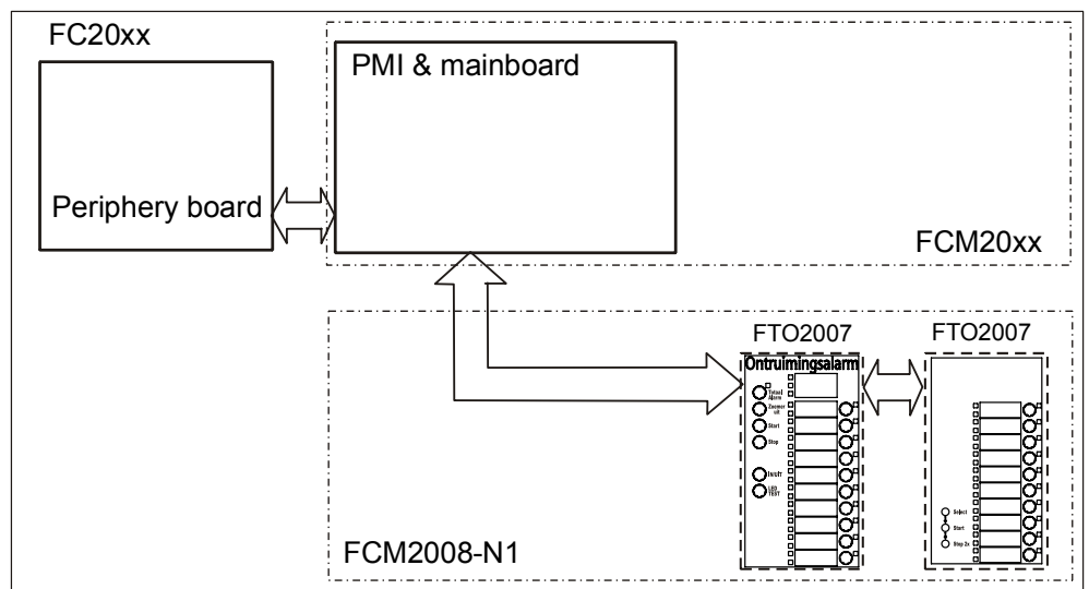
Figure 103: Wiring of integrated EVAC 20-zone display
