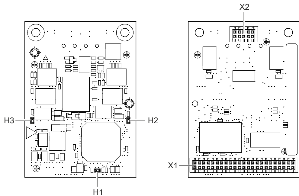
Figure 32: View of network module (SAFEDLINK, CC) FN2010-A1, front and rear panels
