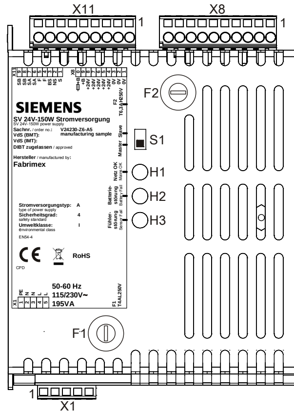
Figure 6: View of power supply (150 W) SV 24V-150W-A5
