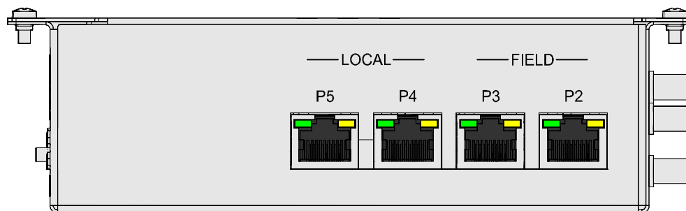
Figure 41: Ethernet connections on the FN2012
