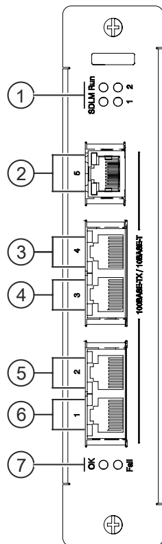
Figure 78: LED indicators of the communication card on the front side
