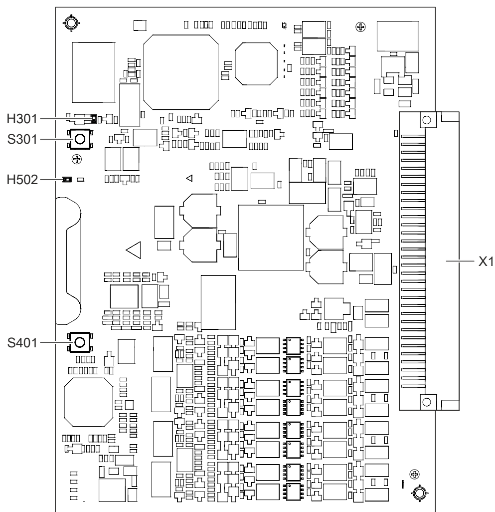
Figure 57: PCB view of the line card (AnalogPLUS) FCL2005
