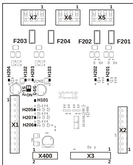
Figure 10: Printed circuit board view FTI2001 fire terminal board
