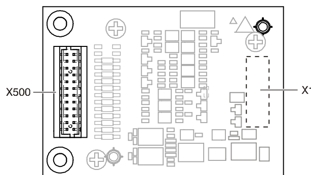
Figure 53: Printed circuit board view of connection module FCA2006-A1
