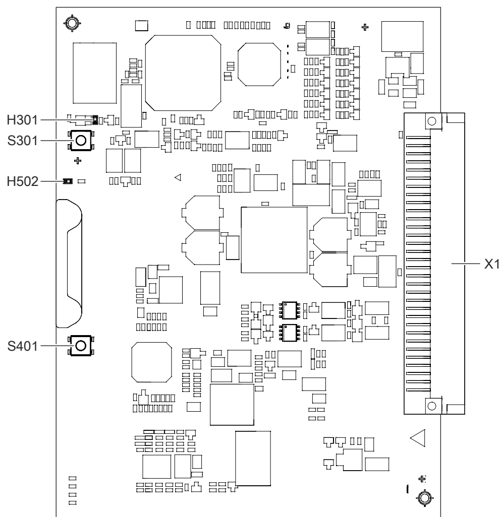
Figure 59: PCB view of the line card (interactive, Ex) FCL2007
