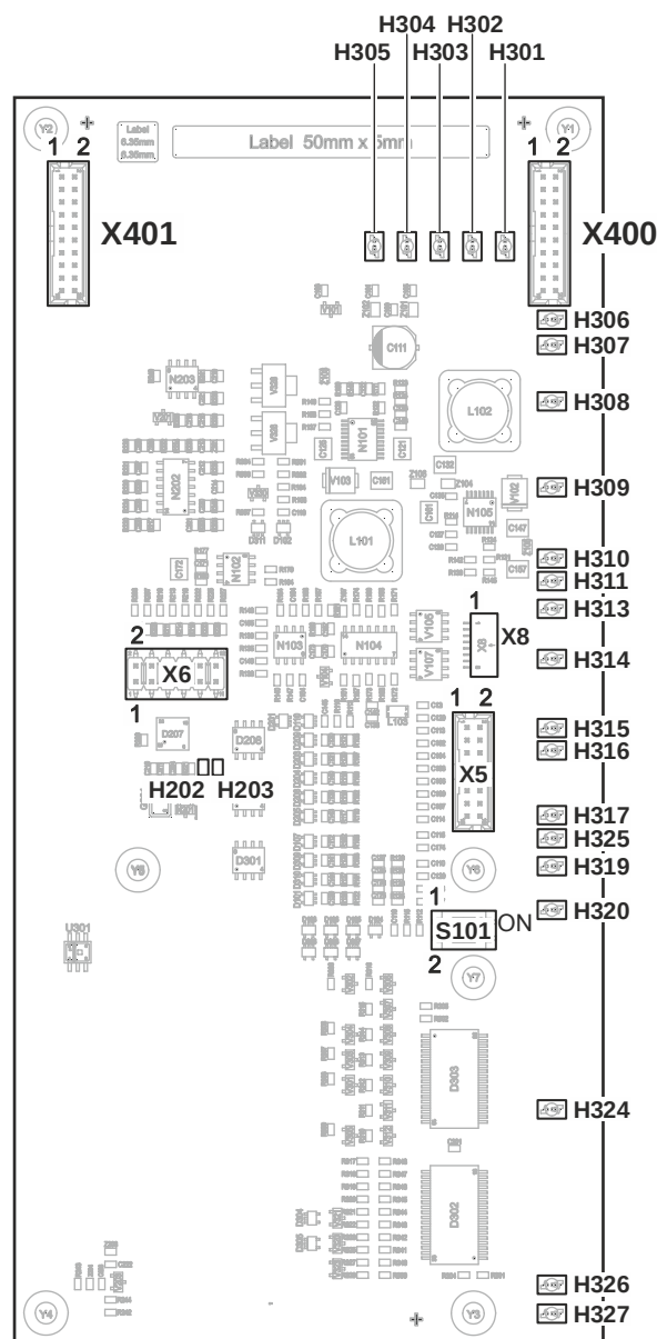
Figure 21: Printed circuit board view, front panel (Touch) FTO2010-A1
