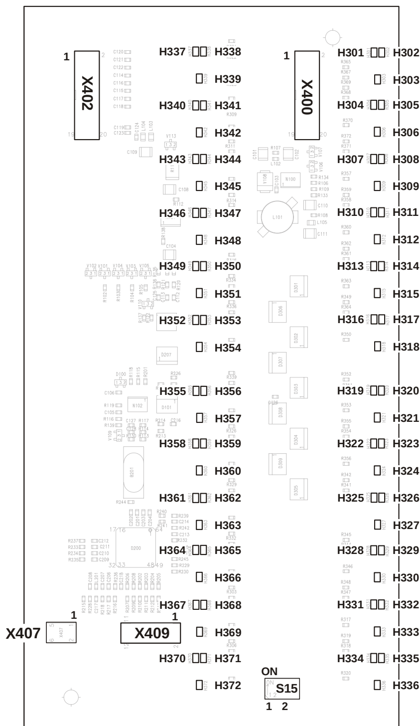
Figure 25: LED module FTO2008-A1, PCB view
