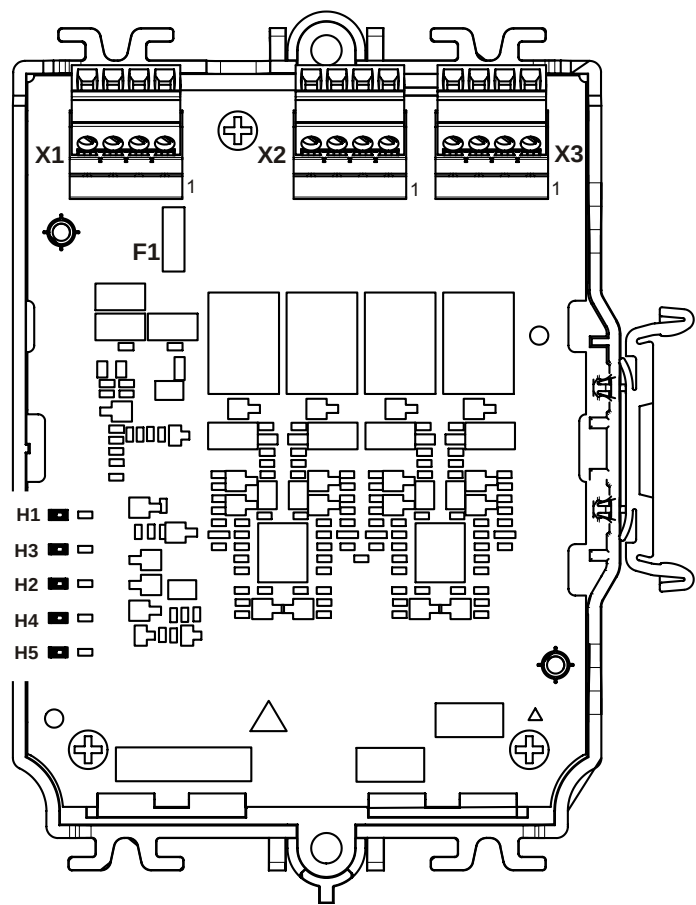
Figure 70: Printed circuit board view of sounder module FCA2005A1
