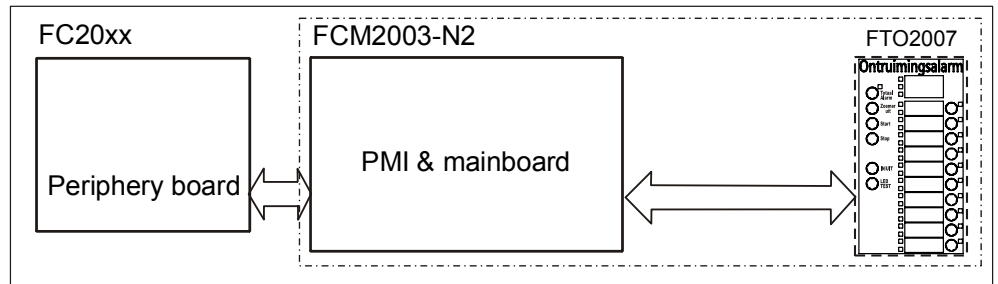
Figure 102: Wiring of integrated EVAC 10-zone display
