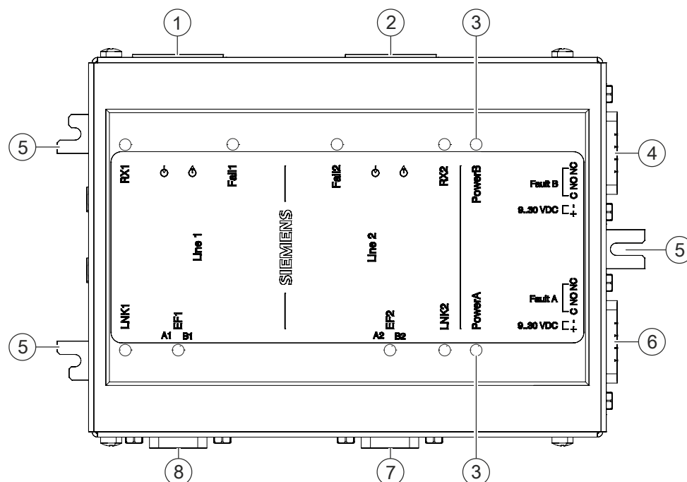
Figure 33: View of fiber optic cable network module (SM/MM)
