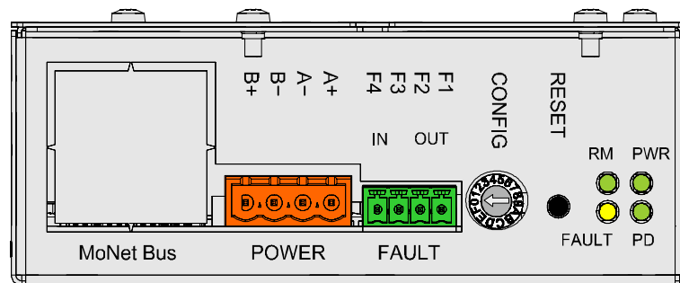
Figure 40: Operating and indication elements on the FN2012
