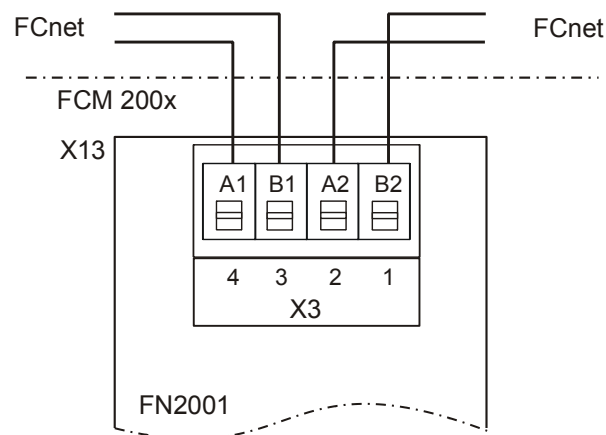
Figure 29: Wiring of 1 network module
