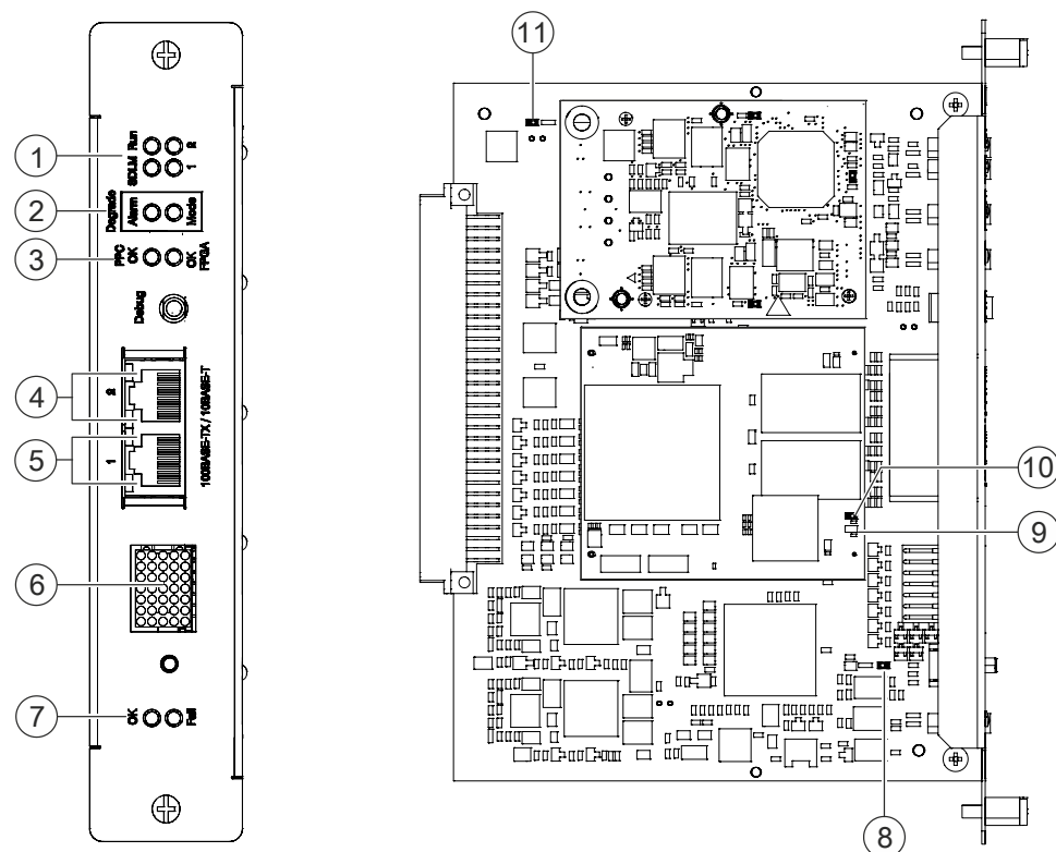
Figure 76: Indicators on ↑ CPU card (FC2080) front side
