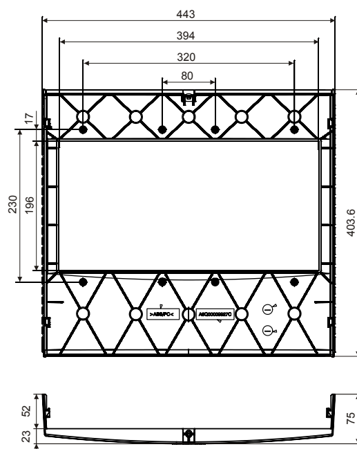
Figure 84: Dimensions of the cover cap
