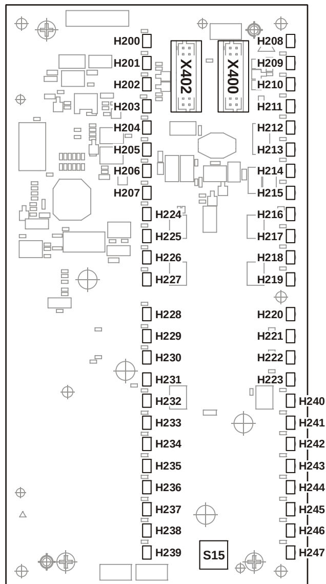
Figure 24: Printed circuit board view of FTO2002-A1
