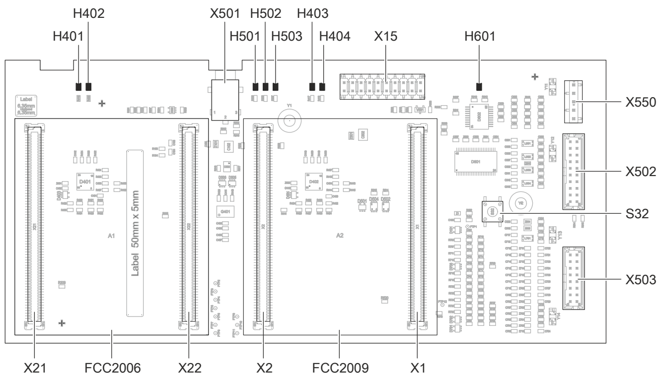
Figure 20: PCB view, carrier for ↑ CPU module FTO2014
