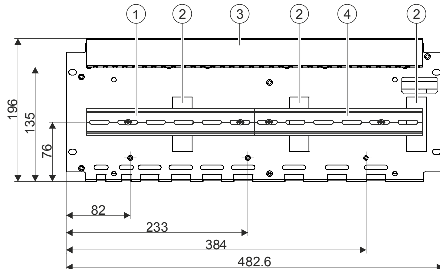
Figure 87: Dimensions of the carrier (19", option) FHA2024-A1
