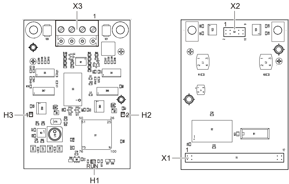
Figure 28: ↑ Network module (SAFEDLINK) FN2001-A1, view of front and rear panels
