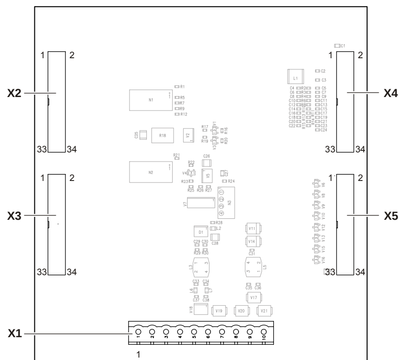
Figure 112: Printed circuit board view of EVAC-NL connector board FTI2002-N1
