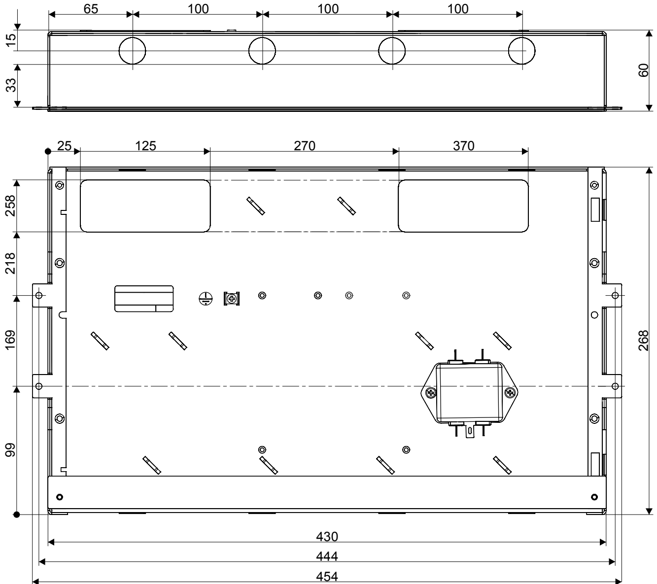
Figure 91: Dimensioned drawing of rear cover (FT2080) FHA2039-A1
