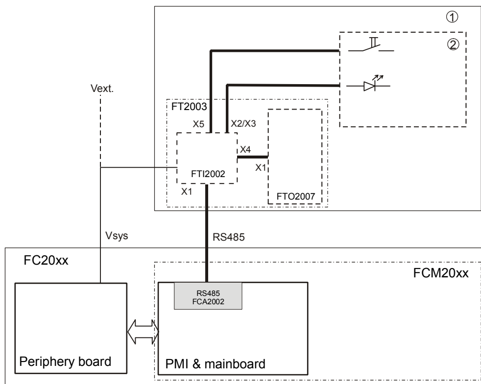
Figure 108: Wiring for EVAC-NL mimic display FT2003-N1
