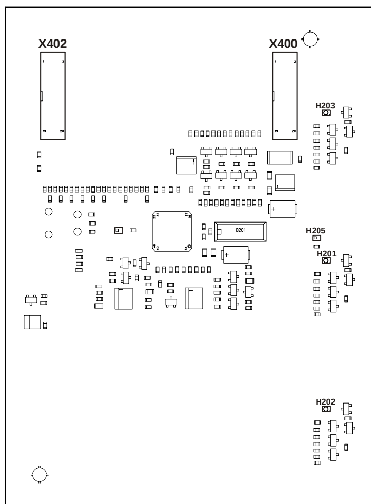
Figure 119: Printed circuit board view FTO2004
