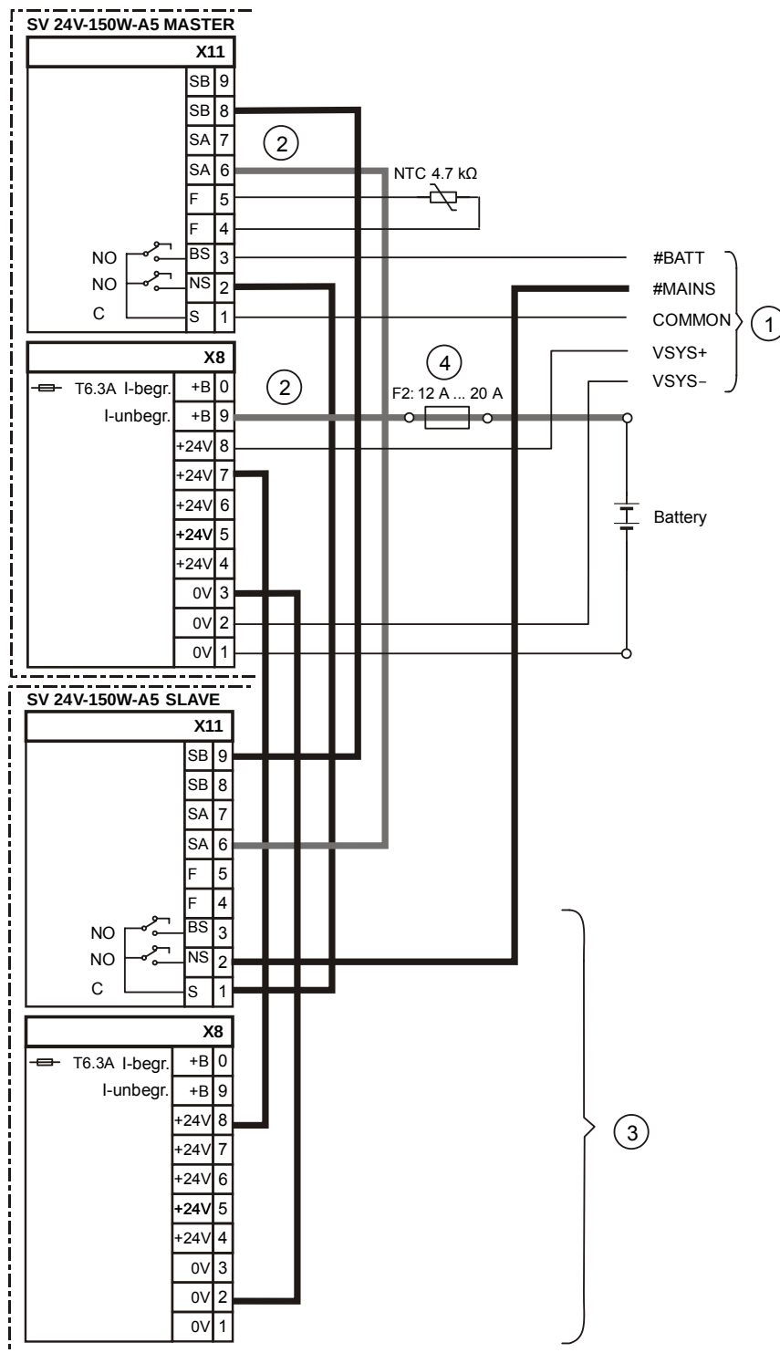
Figure 8: Parallel connection of two power supply units (150 W)-A5
