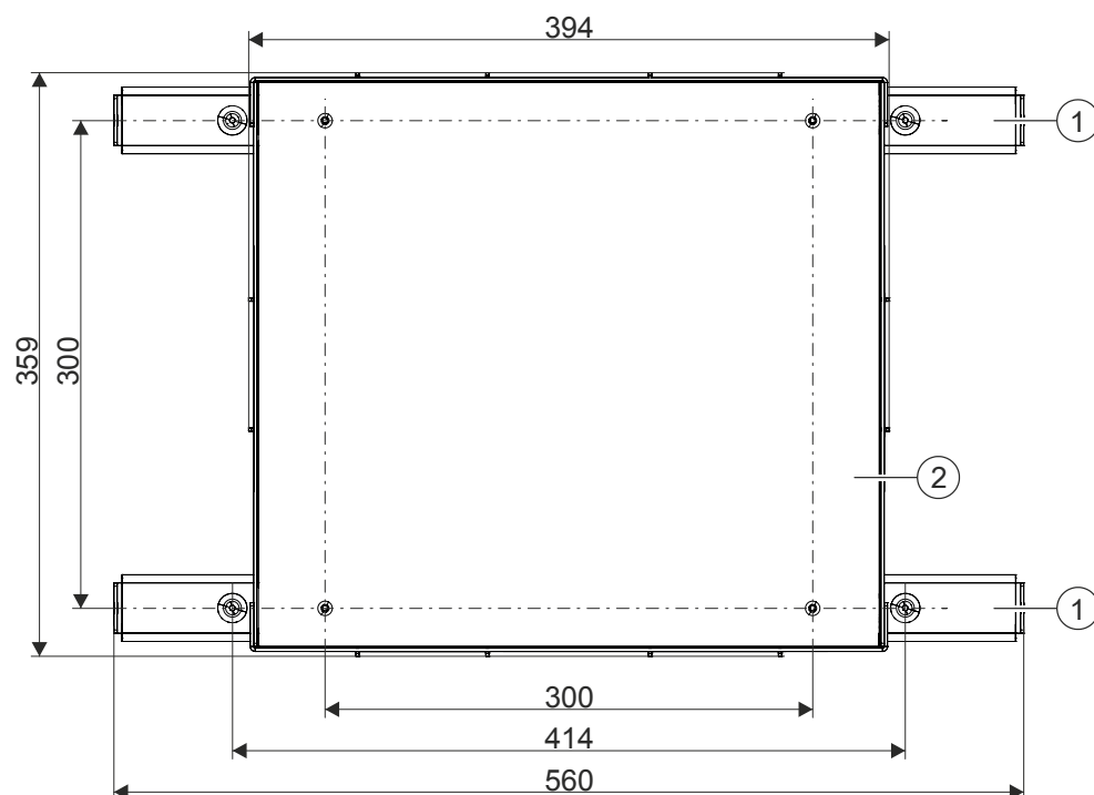
Figure 88: Dimensions of the battery holder complete FHA2021-A1
