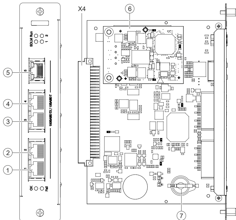
Figure 77: Communication card (FC2080), front and PCB view
