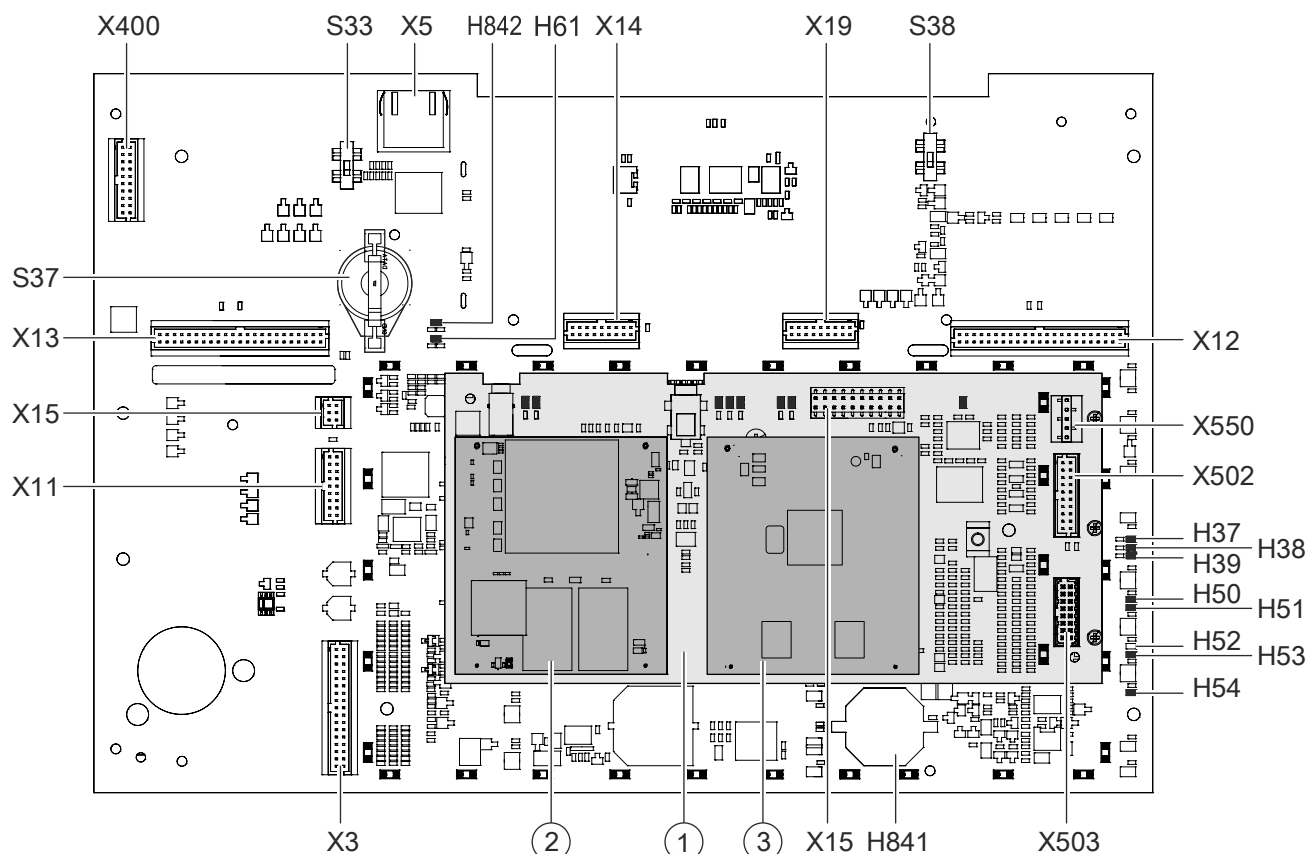
Figure 19: FT2080, PCB view for PMI & mainboard FCM2027 with ↑ CPU module carrier
