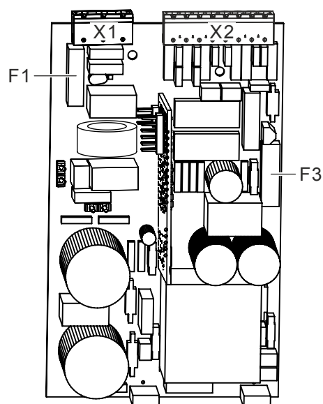
Figure 2: View of PCB FP2015-A1 power supply (70 W)
