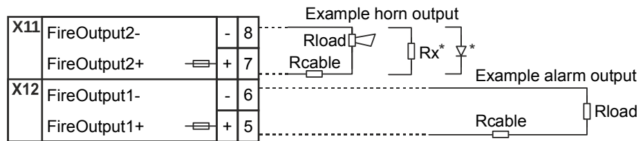
Figure 62: Switching examples for monitored alarm and horn outputs with load resistance monitoring (VdS)
