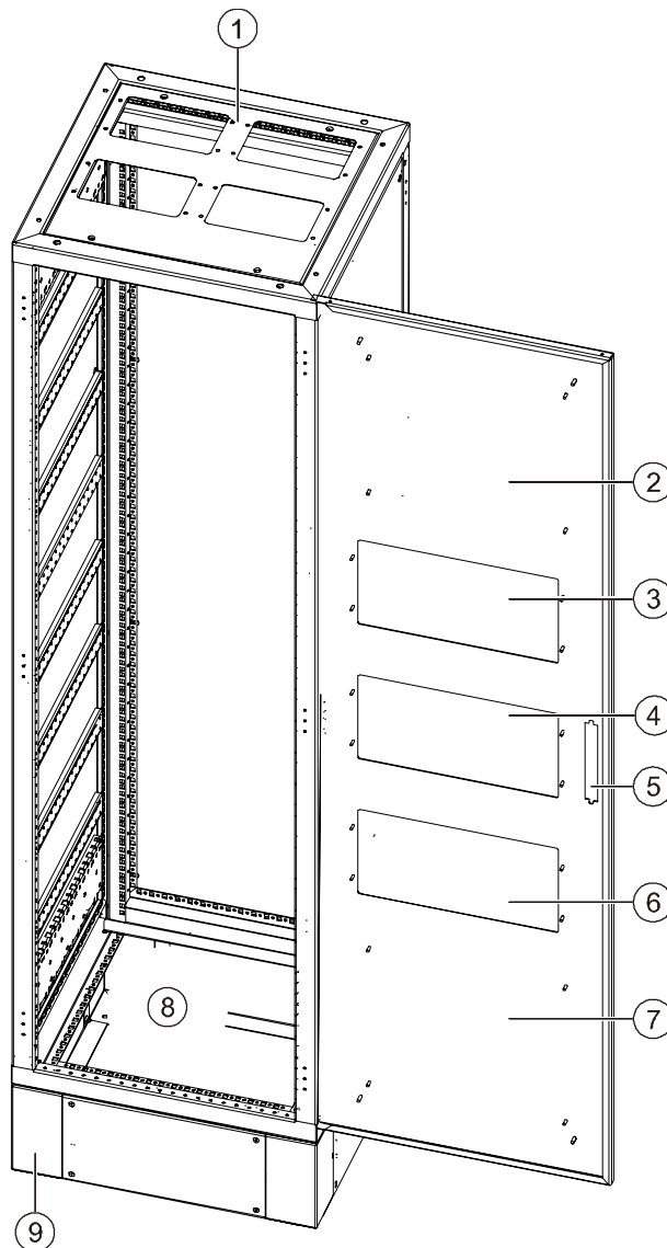
Figure 85: Housing (19" pedestal cabinet)
