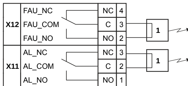
Figure 69: Switching for relays RT Alarm and RT Fault
