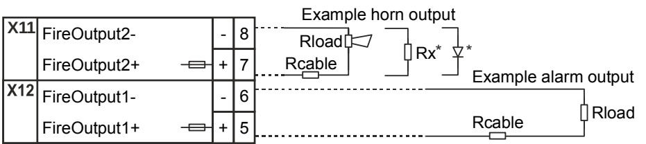
Figure 67: Switching examples for monitored alarm and horn outputs with load resistance monitoring (VdS)
