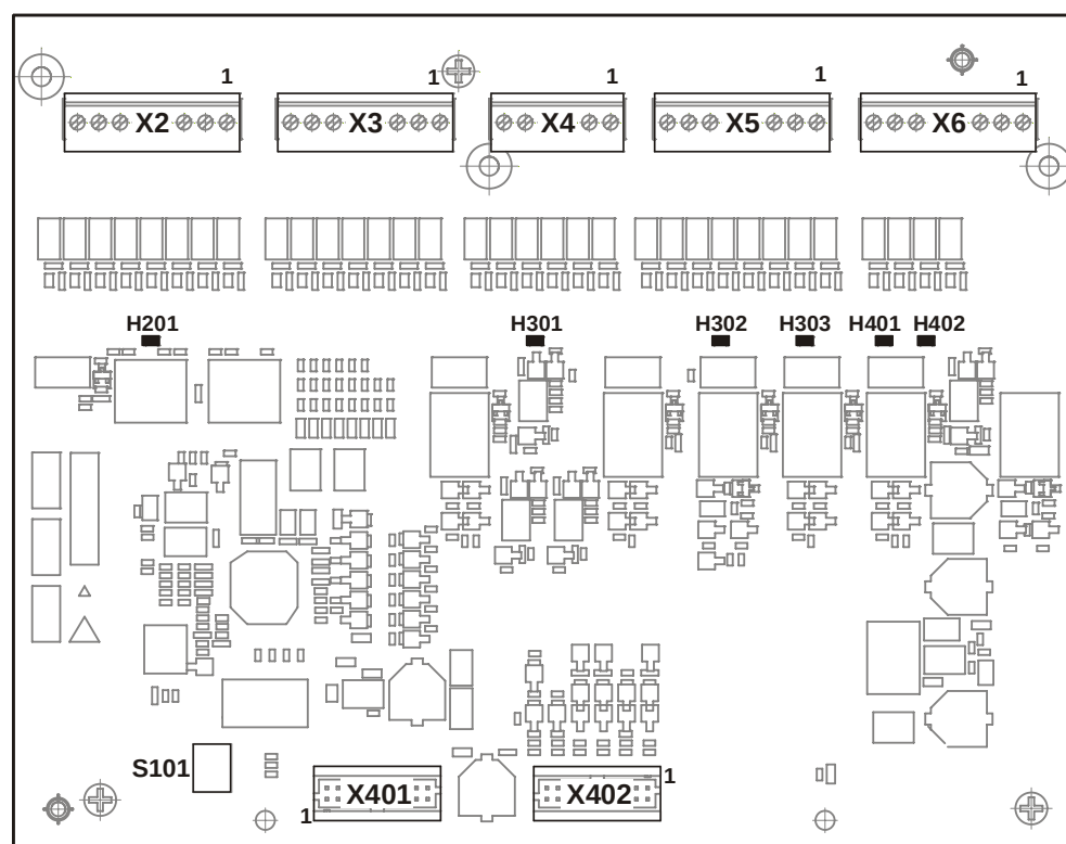
Figure 100: Printed circuit board view of fire brigade periphery module FCI2001-D1
